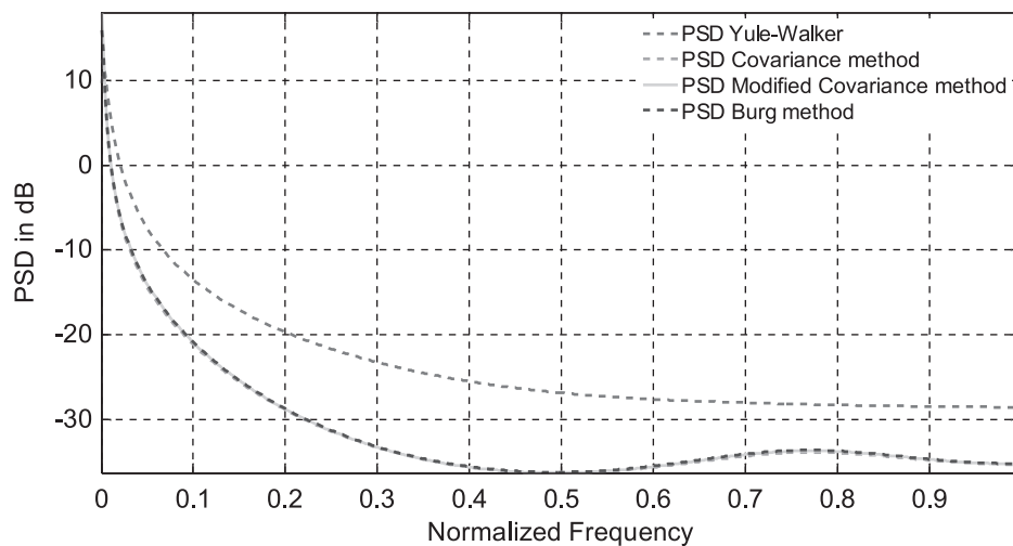
Figure 7. PSD of undisturbed VTEC for all four methods
