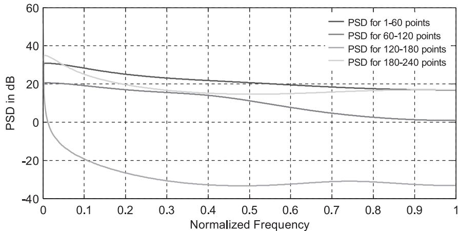
Figure 9: PSD of R_1 for 60 points each
