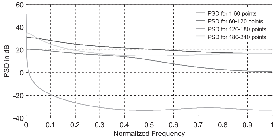
Figure 10: PSD of R_1 for 60 points each
