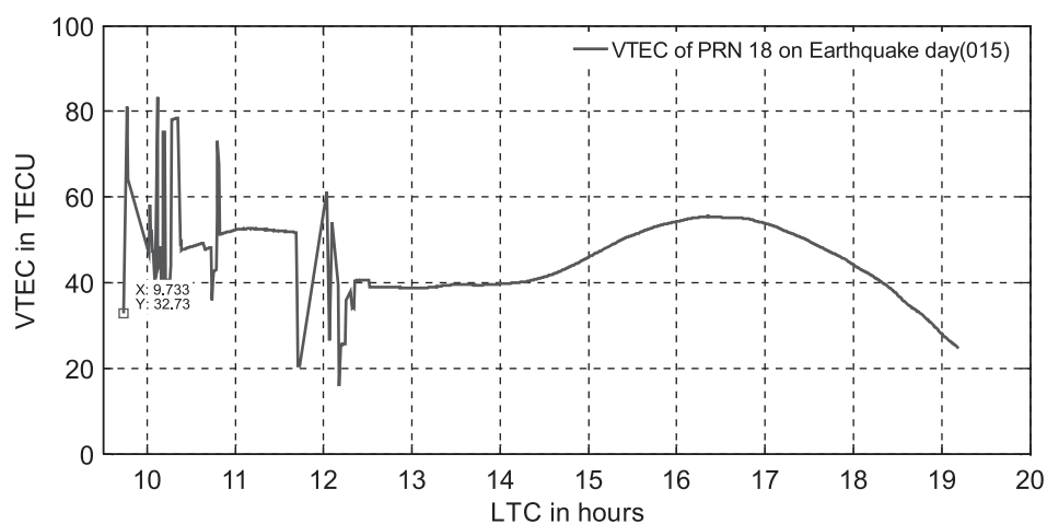
Figure 2: VTEC plot of satellite PRN 18
