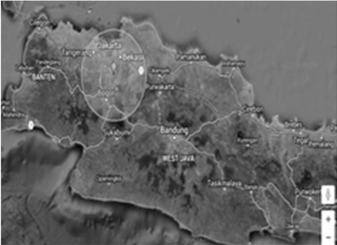
Figure 1: Location map of the earthquake
