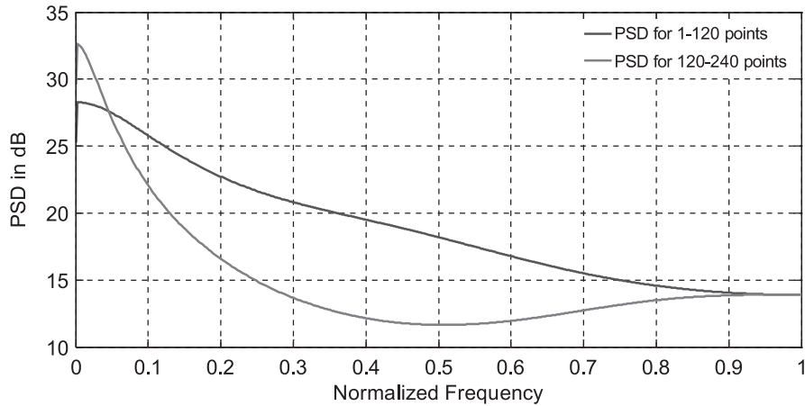
Figure 8: PSD of R_1 for 120 points each
