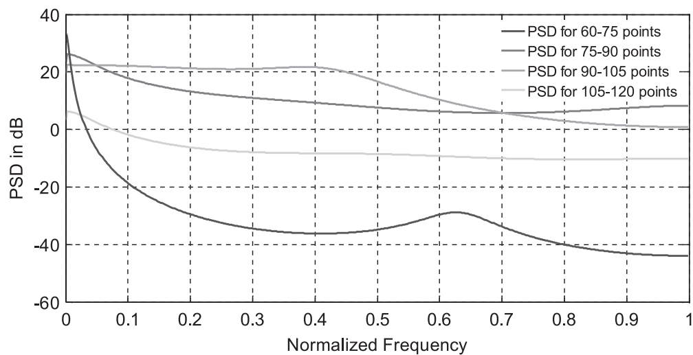
Figure 14: PSDs for second four sets of R_1 with 15 points
