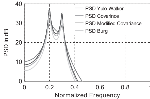
Figure 3: PSD's of Yule-walker, Covariance, Modified Covariance and Burg methods for the Synthetic Signal
