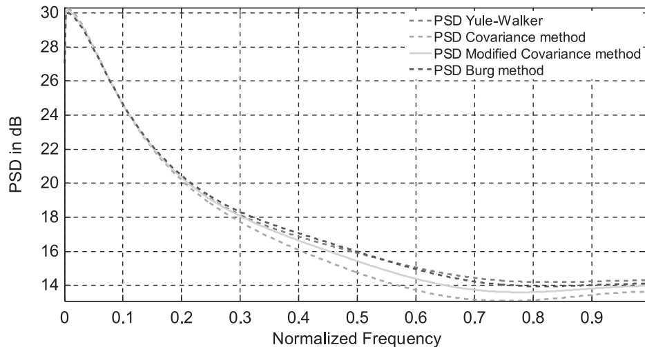
Figure 6. PSD of disturbed VTEC for all four methods
