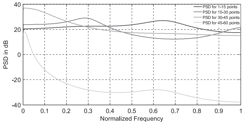
Figure 13: PSDs for first four sets of R_1 with 15 points
