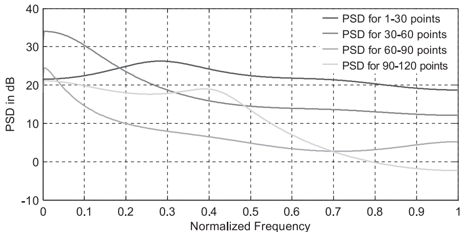
Figure 11: PSDs of R_1 for first four sets 30 points
