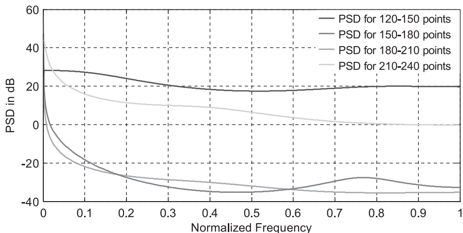
Figure 12: PSDs for second four sets of R_1 with 30 points
