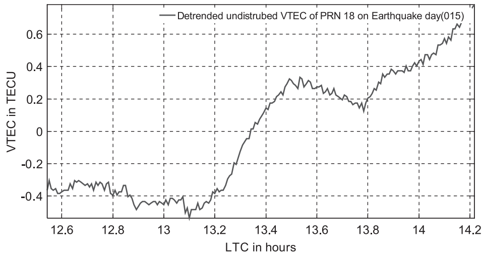
Figure 5. Detrended R_2 data
