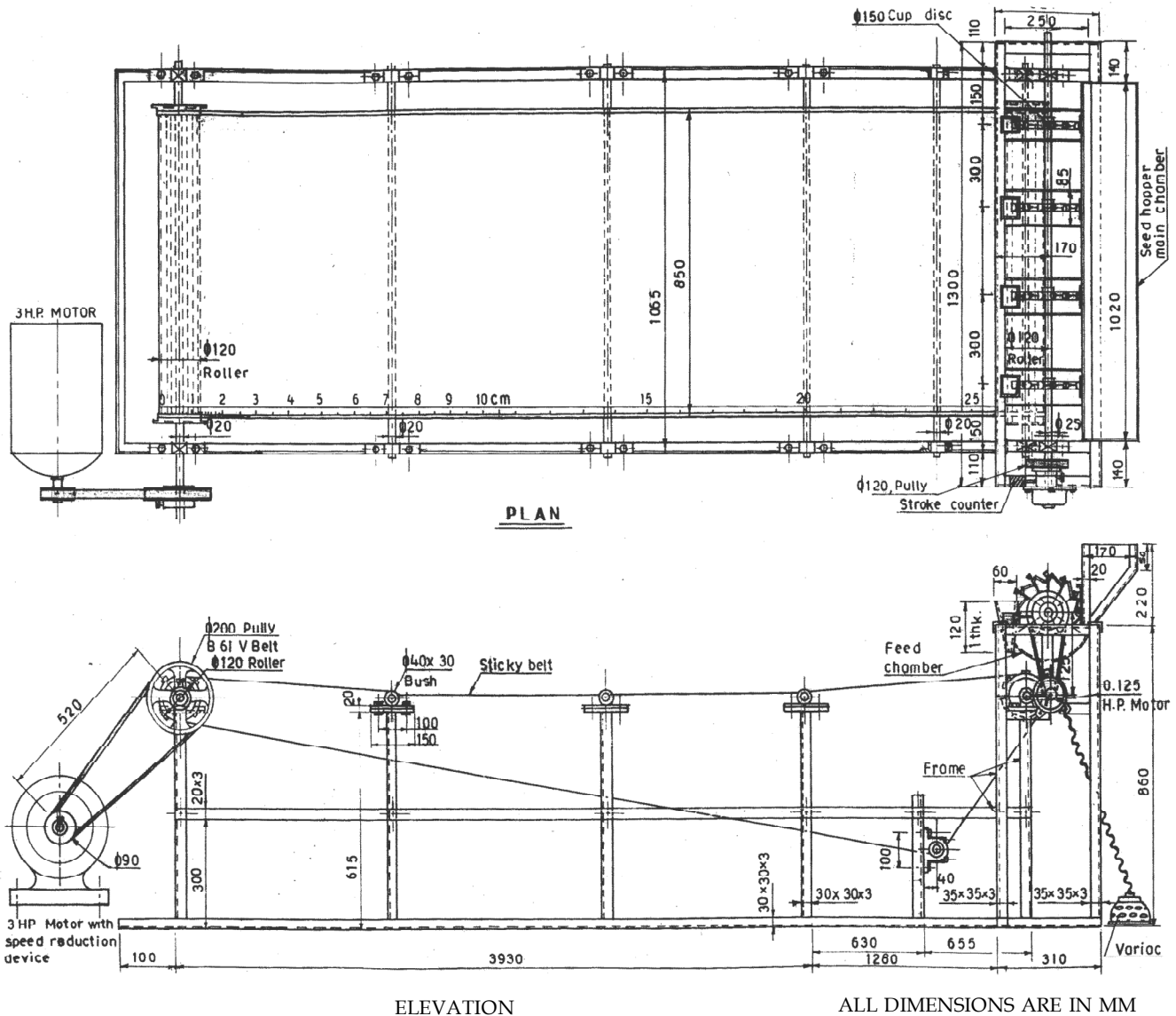
Figure 2: Test Rig for Performance Evaluation of Cup Feed Metering Device
