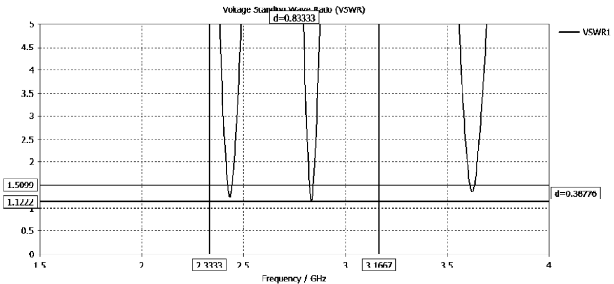
Figure 11: VSWR of the proposed patch
