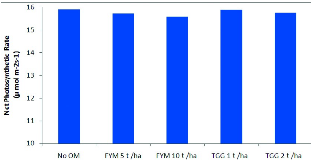
Figure 4: Effect of different organic manures and fertilisers on Net photosynthetic rate of FCV tobacco (Var. Kanchan) in irrigated Alfisols
