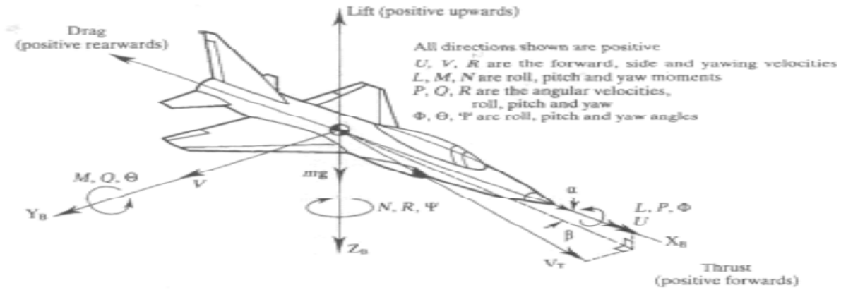
Figure 1: Aerodynamic forces, moments and velocity components
