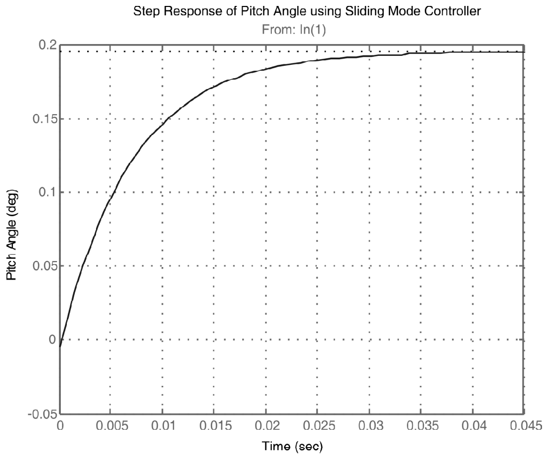
Figure 4: Response of system using SMC
