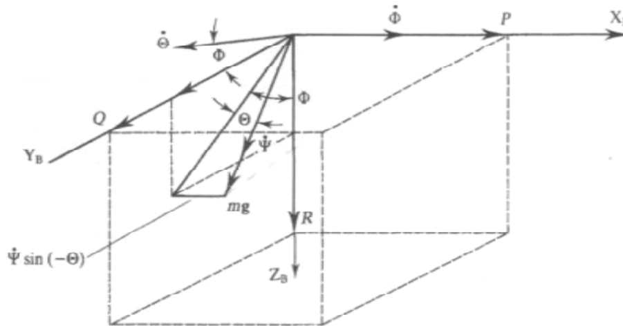
Figure 2: Angular orientation and velocities of gravity vector
