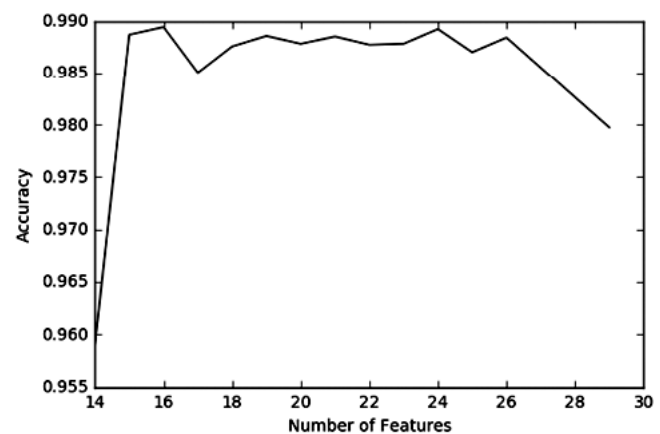
(b) Accuracy vs Features for KDD Cup 99
