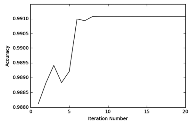
(b) Accuracy vs Iteration for KDD Cup 99
