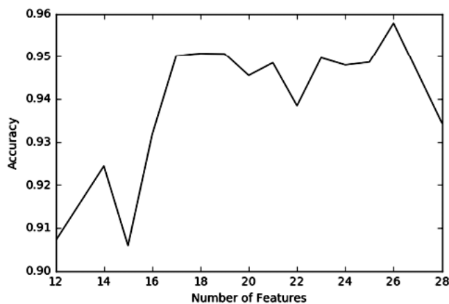
Figure 2: (a) Accuracy vs Features for NSL-KDD
