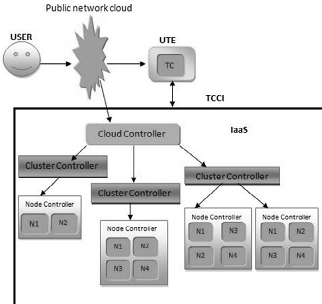
Figure-3: Trust model
