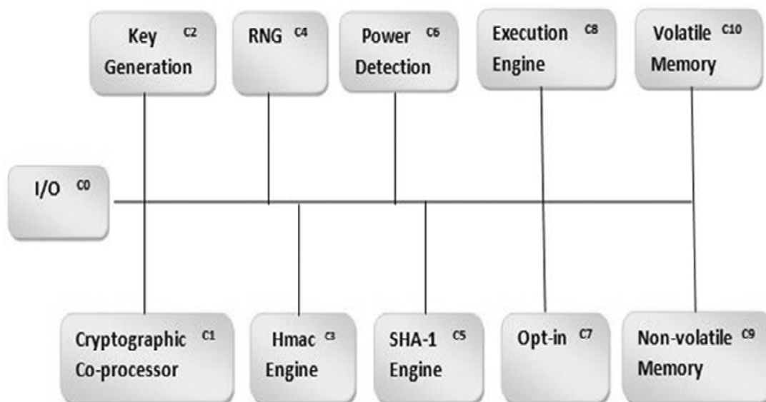
Figure 2: TPM Structure
