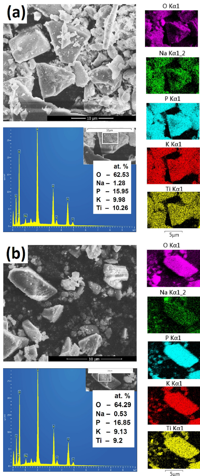
Figure 5. SEM images, EDS analysis, and mapping of the elements for separate crystals with different morphologies: a) K_{2-x}Na_xTi_2(PO_4)_3 ( x = 0.22-0.26 ) solid solutions and b) KTiP_2O_7 .
