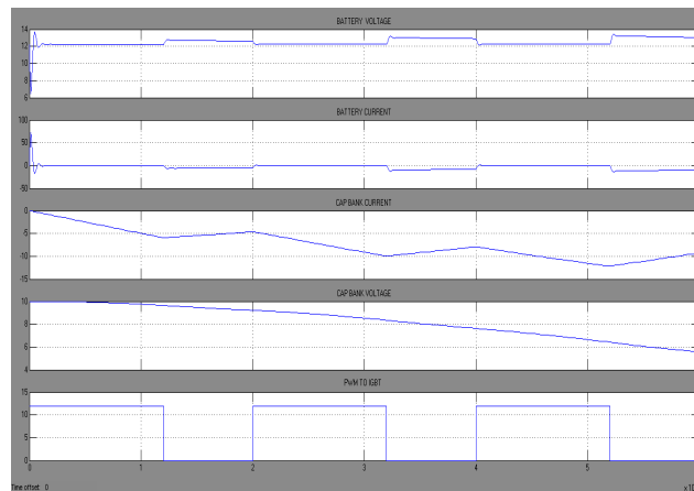
Figure 6: Waveform for Boost Cycle (Acceleration)
