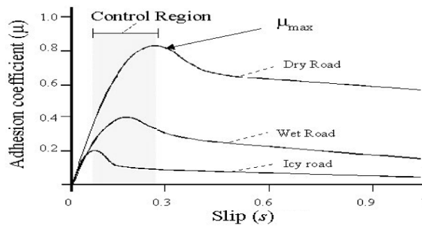
Figure 1: \mu -s sample characteristics
