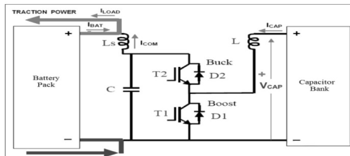
Figure 2: Regenerative braking circuit
