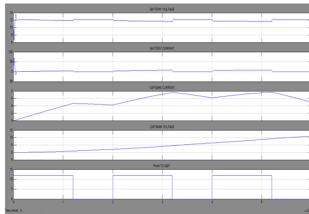
Figure 5: Waveform for Buck Cycle (Deceleration)
