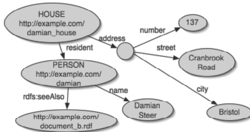
Fig. 2. RDF Graph Example [31]
