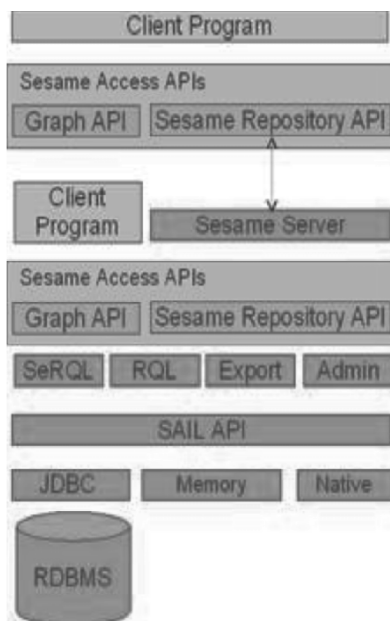
Fig. 5. Sesame Architecture[27]
