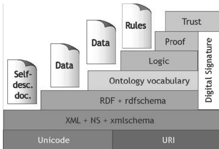
Fig. 1. The Semantic Web Layered Structure [30]
