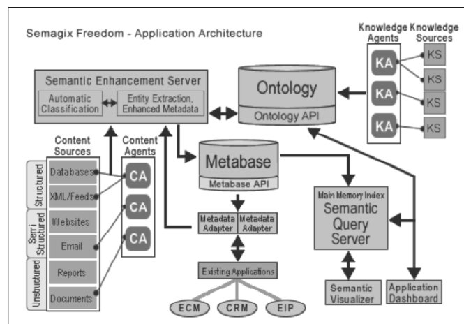
Fig. 4. The Architecture of Semagix Freedom[9]
