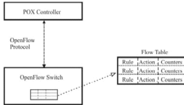
Figure 2: Open Flow Switch
