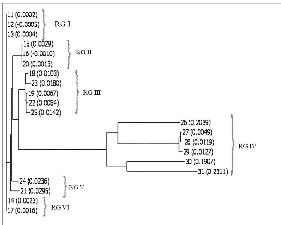
Figure 2: Dendrogram representation of a Phylogenetic tree and RGA groups (RG I-VI) formed based on multiple sequence alignment of selected RGA sequences listed in Table 2 with GenBank accession numbers
