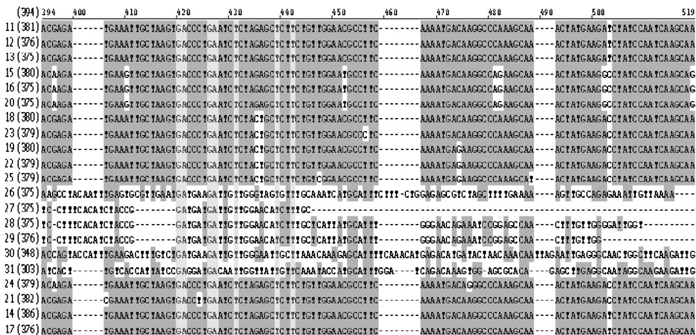
Figure 1: Multiple alignment of selected RGA sequences using Align X program and nucleotide changes in RGA sequences are shown without colour
