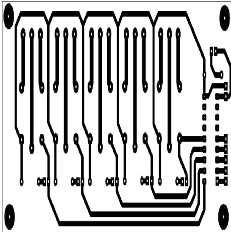
Figure 7: PCB Design Relay layout
