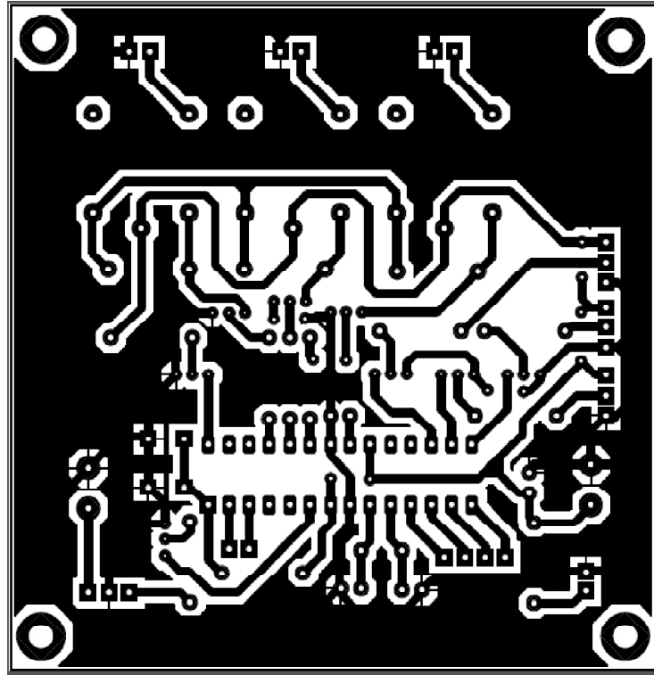
Figure 6: PCB Design of control section
