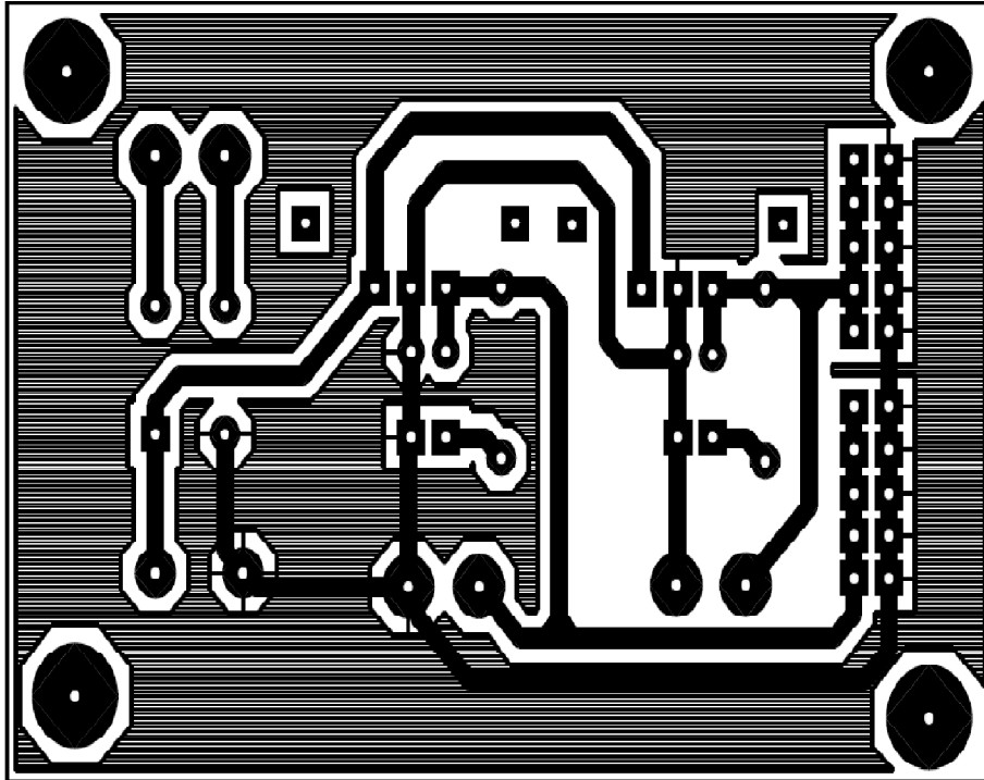
Figure 8: PCB Design Power supply
