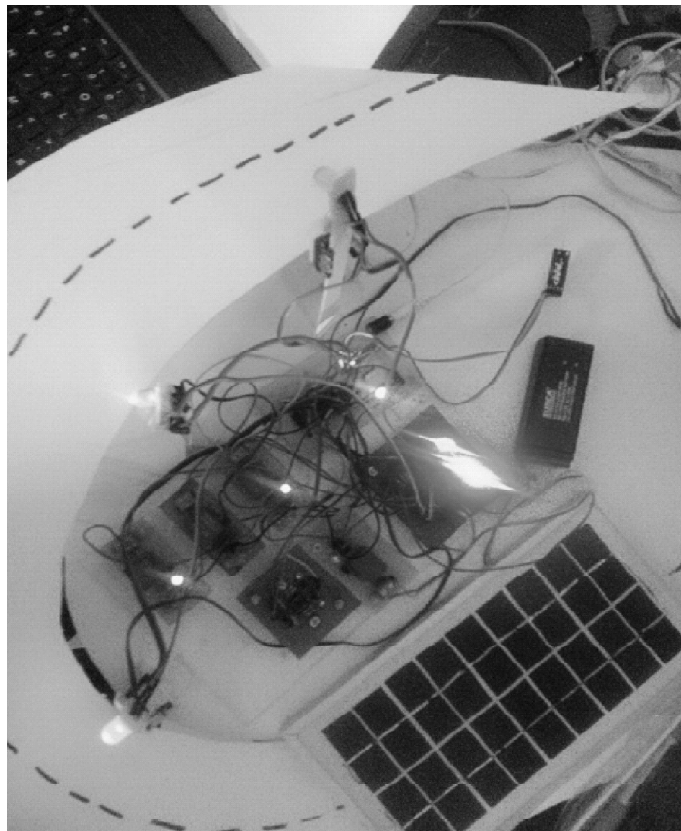
Figure 9: Hardware Model
