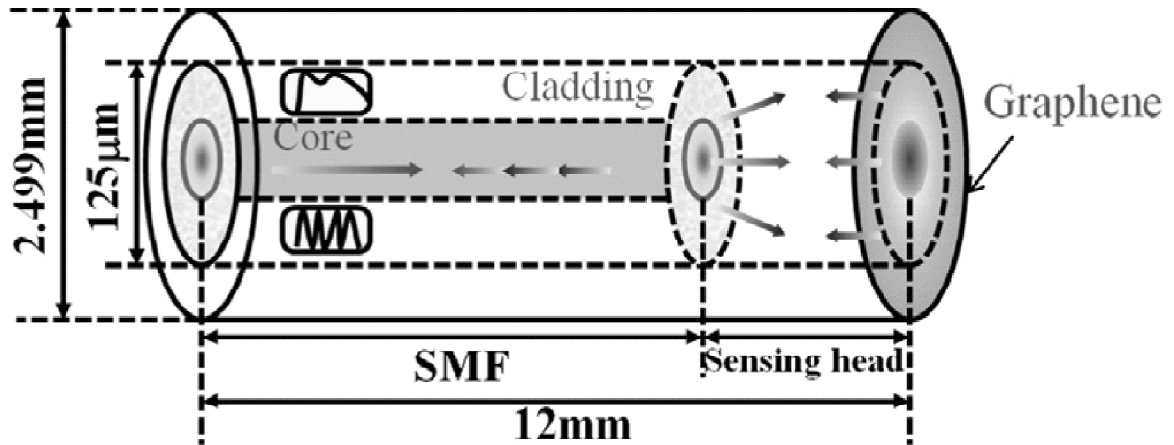
Figure 6: The schematic diagram of the sensor head [128]
