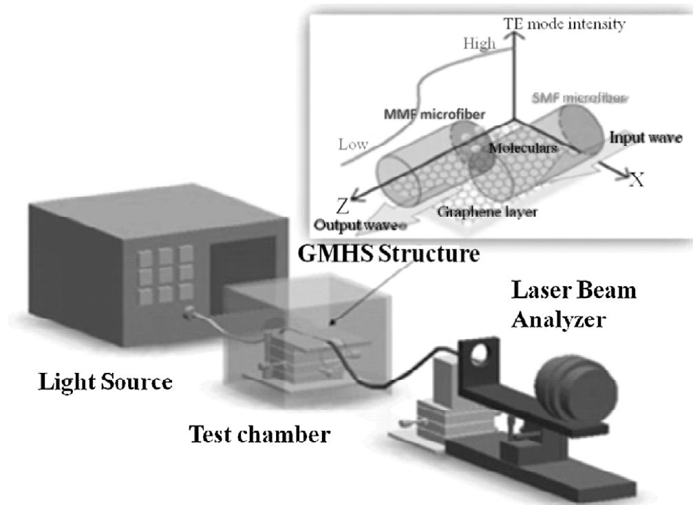
Figure 7: Experiment setup of hybrid waveguide gas sensor [129]
