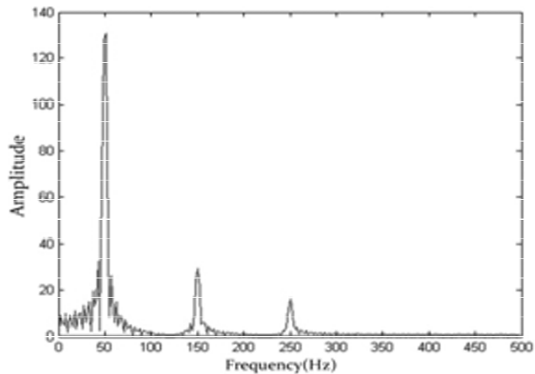
Figure 4: FFT of input signal (Fundamental more prominent but harmonics present)
