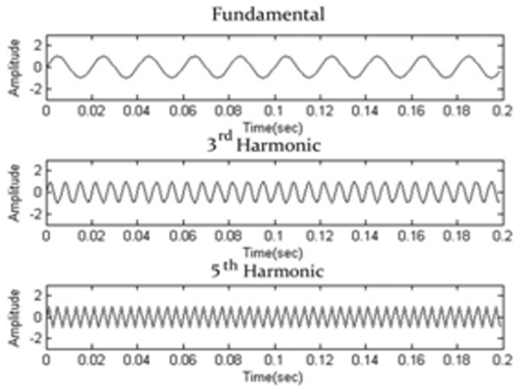
Figure 2: Input signal (Fundamental + Harmonics)
