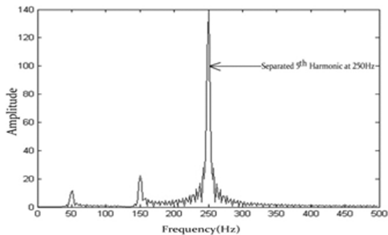
(b) Separation of 5 th harmonics at 250Hz
