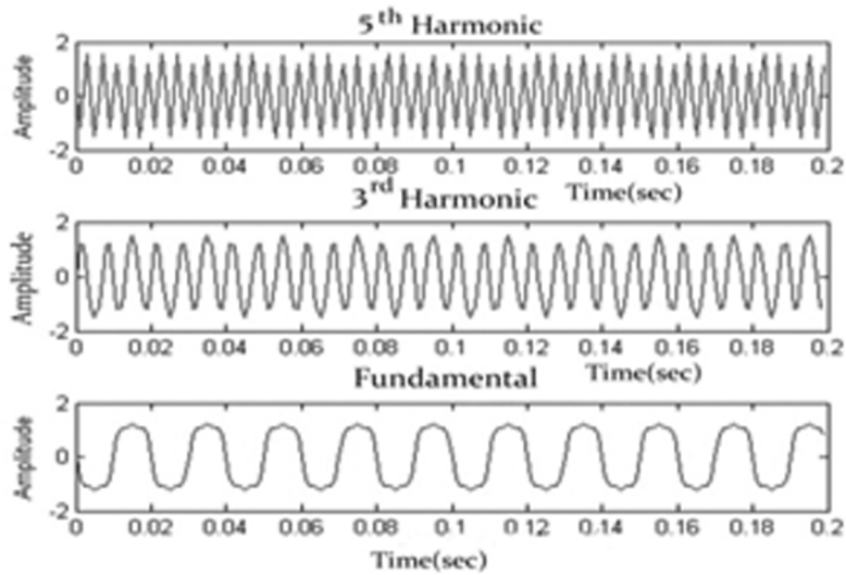
Figure 3: Separated signals
