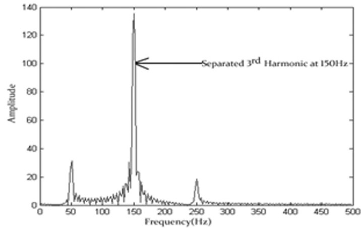
(a) Separation of 3 rd Harmonics at 150Hz
