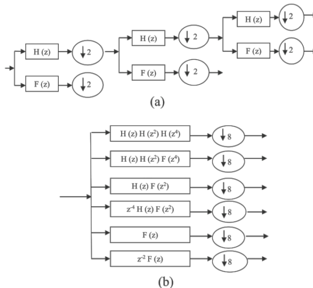
Figure 1. 3-scale filter banks (a) DWT (b) Equivalent Slantlet representation
