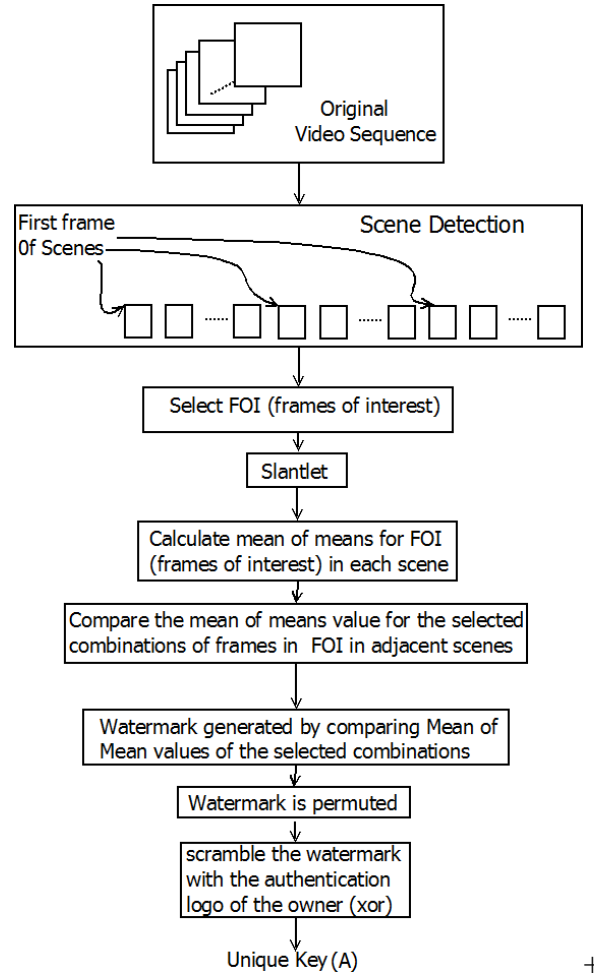
Figure 3. Proposed zero watermarking algorithm block diagram
