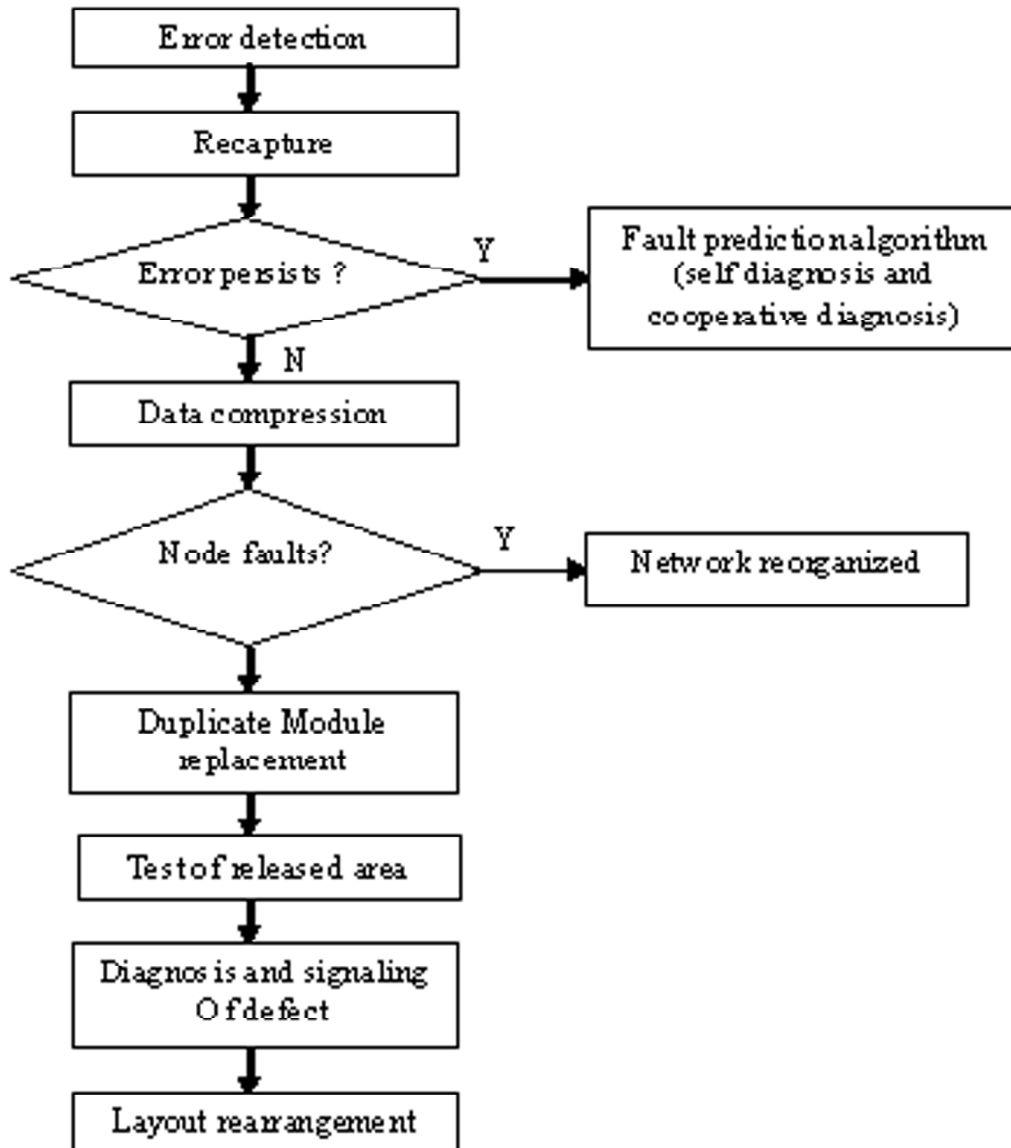
Figure 6: Working flowchart
