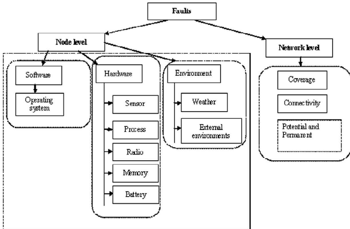
Figure 2: Fault Model
