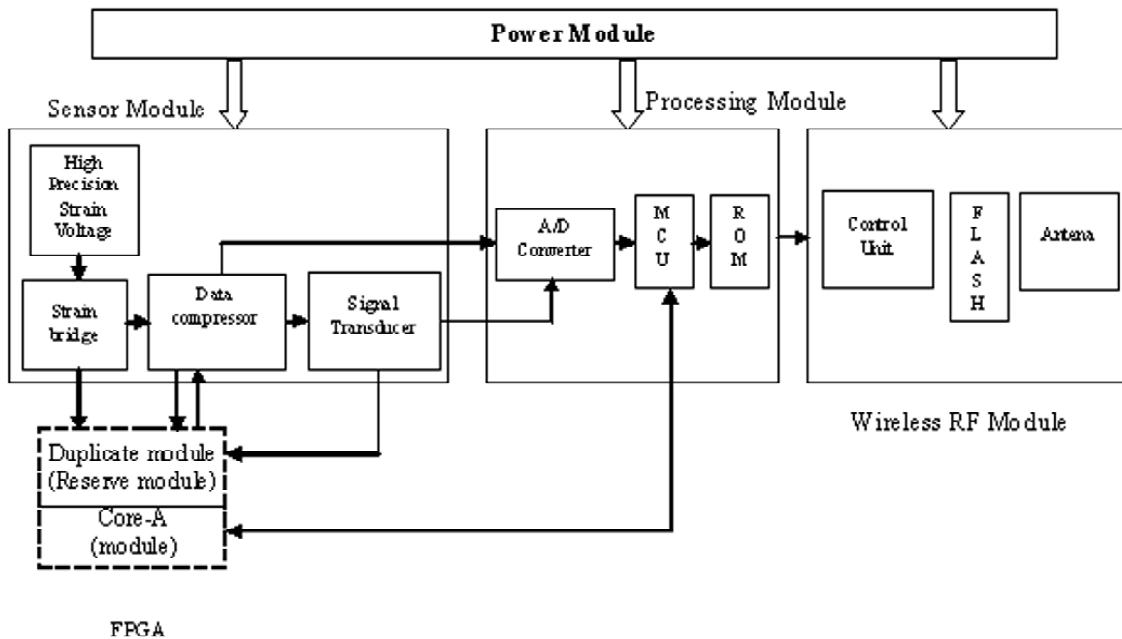
Figure 5: Proposed method of FPGA based self-healing WSN node design
