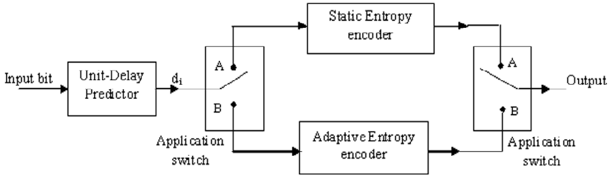
Figure 1: Block diagram of Entropy encoding algorithm
