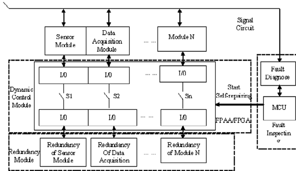
Figure 4: Redundancy based self-healing WSN node design
