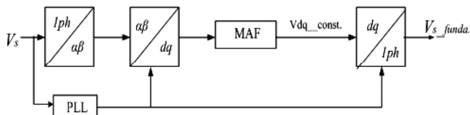
Figure 2: Fundamental positive sequence component extraction
