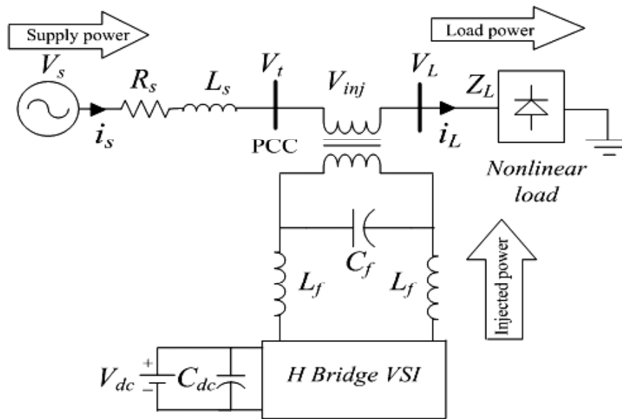
Figure 1: Single phase system configuration with DVR
