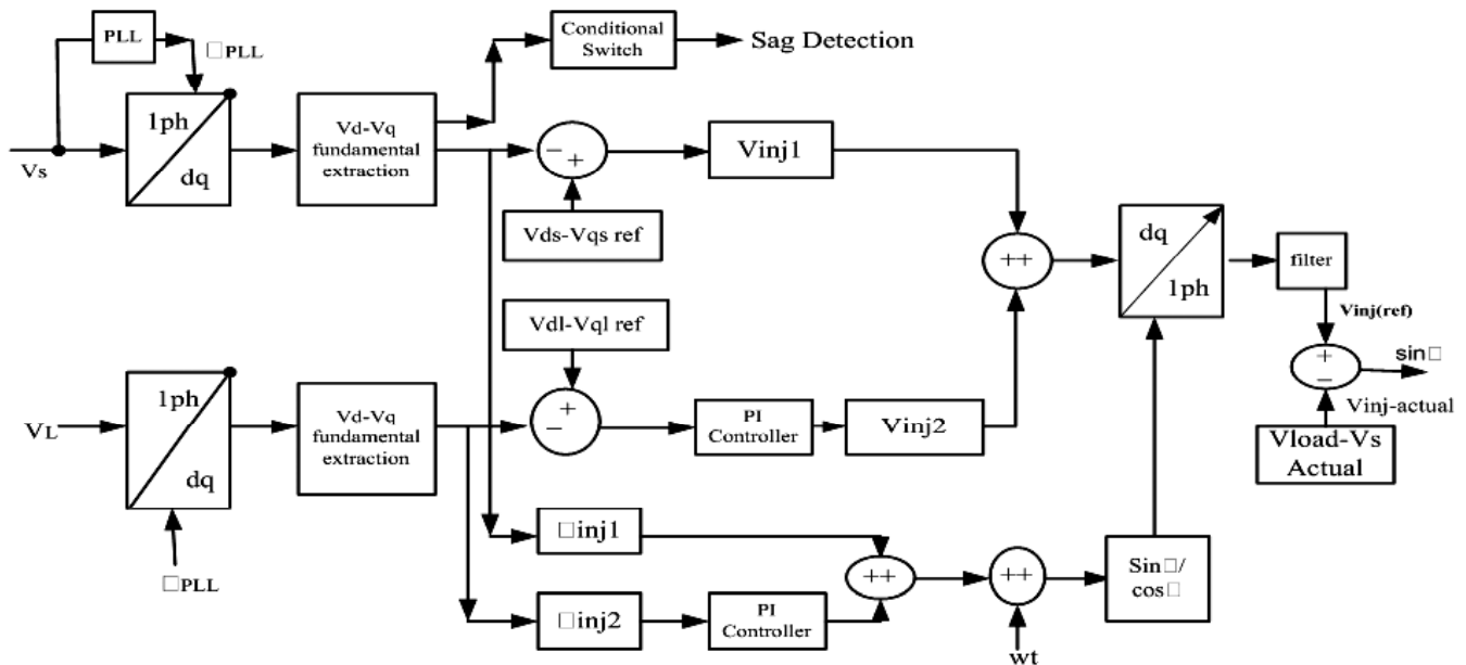
Figure 4: MATLAB based model of proposed control method
