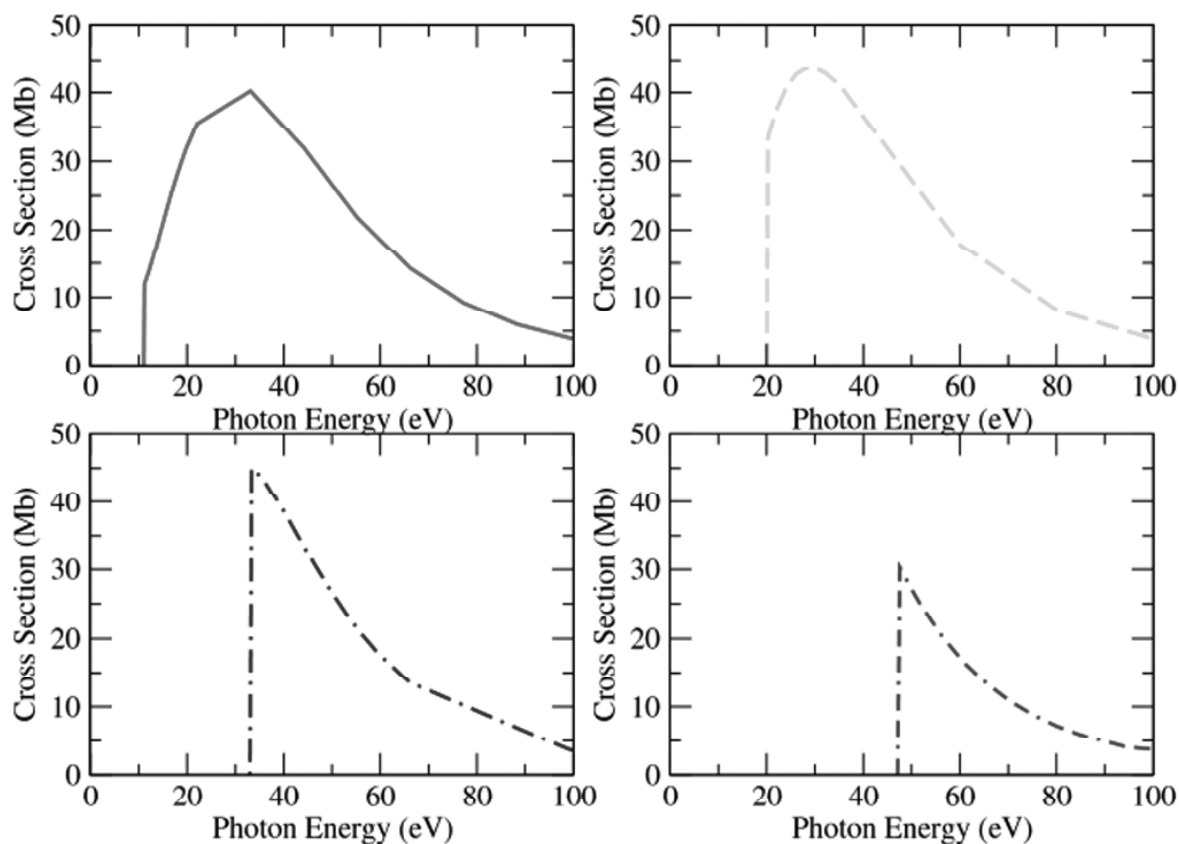
Figure 5. Photoionization of Au: 5d^{10}6s \rightarrow 5d^96skl , solid line, photoionization of \text{Au}^+ : 5d^{10} \rightarrow 5d^9kl , dashed line, photoionization of \text{Au}^{2+} : 5d^9 \rightarrow 5d^8kl , dot dashed line, photoionization of \text{Au}^{3+} : 5d^8 \rightarrow 5d^7kl , dot double dashed line ( 1.0 \text{ Mb} = 1.0 \times 10^{-18} \text{ cm}^2 ).
