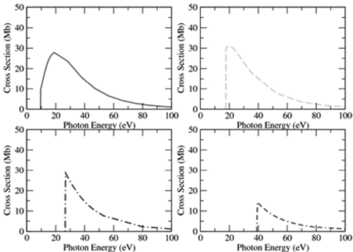
Figure 1. Photoionization of Re: 5d^5 6s^2 \rightarrow 5d^4 6s^2 kl , solid line, photoionization of Re^+ : 5d 5s \rightarrow 5d 4s kl , dashed line, photoionization of Re^{2+} : 5d^5 \rightarrow 5d^4 kl , dot dashed line, photoionization of Re^{3+} : 5d^4 \rightarrow 5d^3 kl , dot double dashed line (1.0 Mb = 1.0 \times 10^{-18} cm 2 ).
