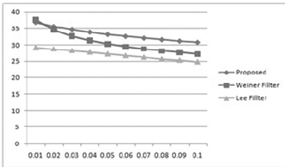
Figure 2: Comparison in terms of PSNR
