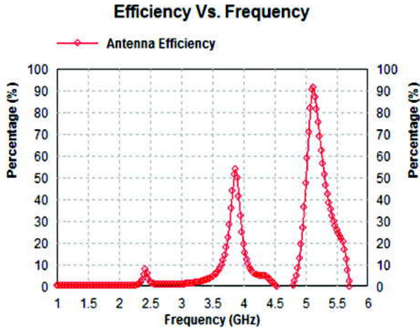
Figure 6: Antenna efficiency of proposed antenna
