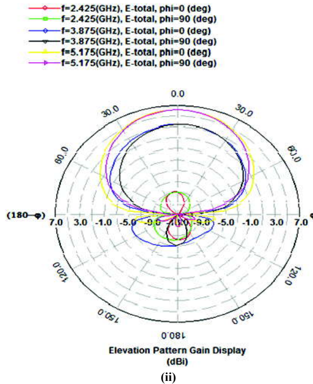
Figure 7. 2D radiation pattern of proposed antenna (i) for 2.5 GHz (ii) for 2.42,3.87and 5.2 GHz
