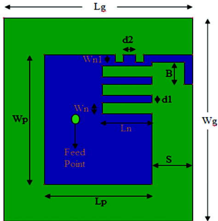
Figure 2: Geometry of proposed antenna
