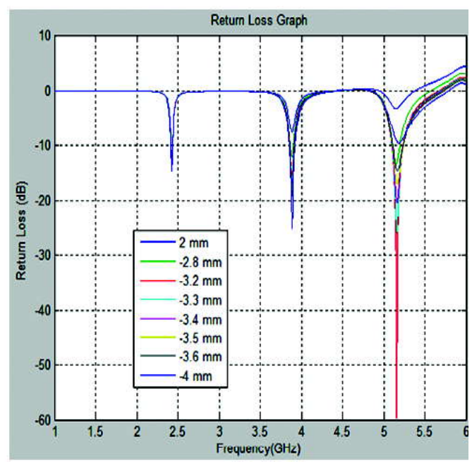
Figure 11: Return Loss for different value of feed position
