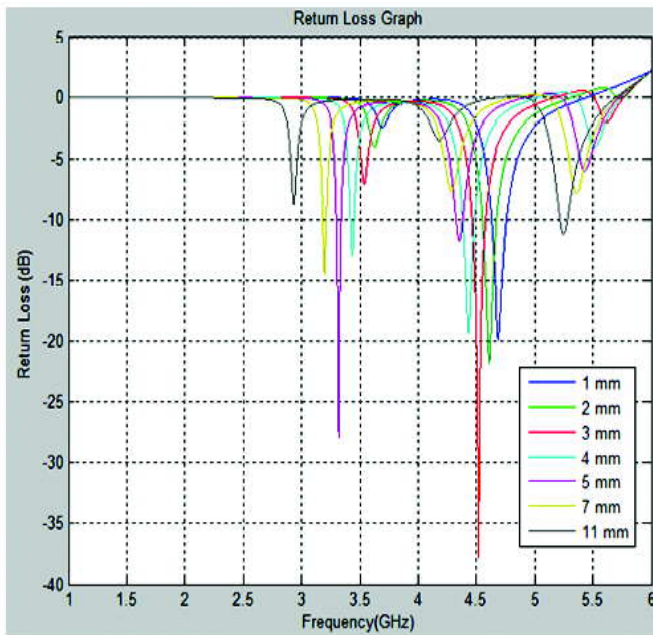
Figure 10: Return loss with the variation in width of band
