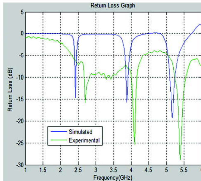
Figure 4. Return loss of proposed antenna
