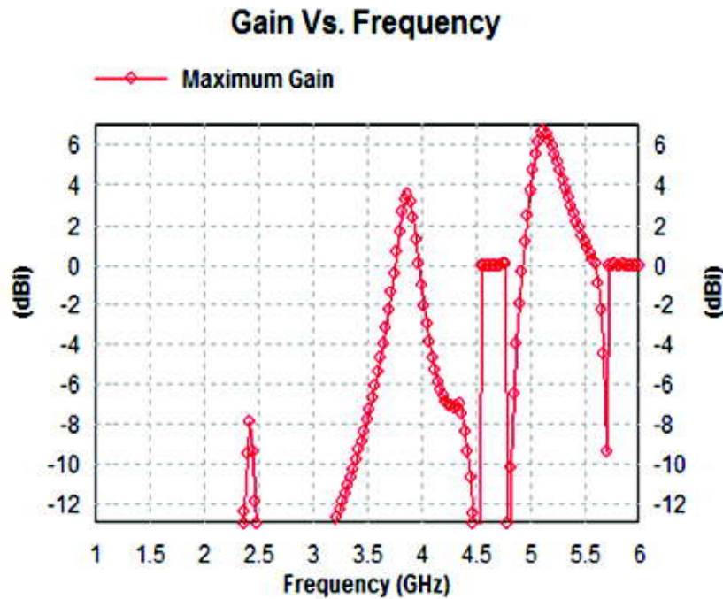
Figure 5: Gain of proposed antenna
