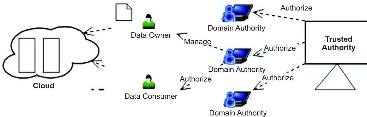
Figure 3: Proposed approach implementation procedure
