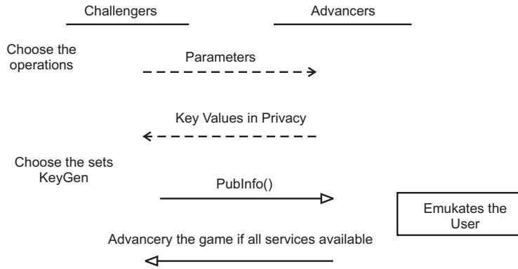
Figure 4: TTKM procedure with group sharing in cloud
