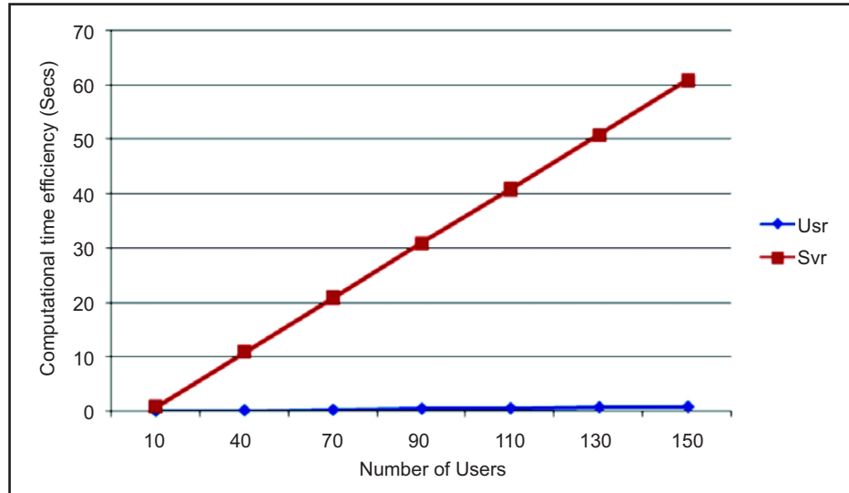
Figure 7: Computational time at Usr and Svr with group users in file computation
