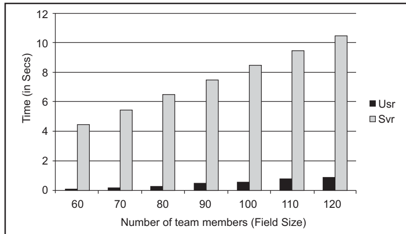
Figure 6: Dimensionality based data sharing in cloud with field size with group members
