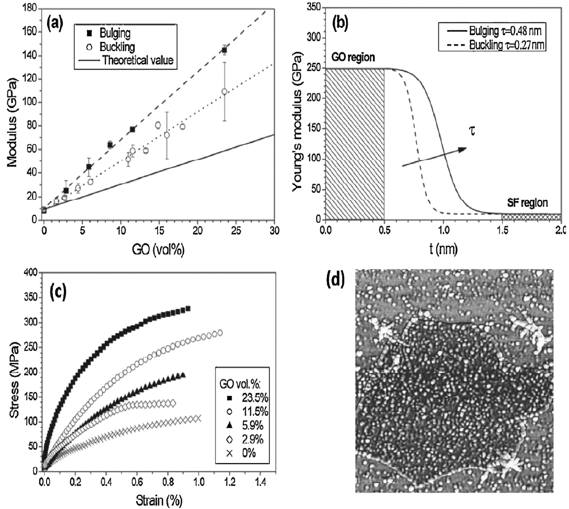
Figure 18: (a) Elastic moduli of the graphene oxide-silk fibroin nanocomposite versus GO content and (b) the interphase modulus transition model (distribution from modulus across GO-silk region). (c) Representative stress-strain curves. (d) AFM phase image of the silk fibroin adsorbed on graphene oxide flake [64]. Copyright 2013. Reproduced with permission from John Wiley & Sons Inc.
