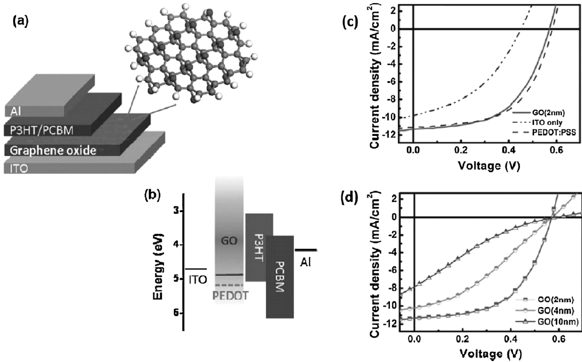
Figure 23: Device schematic (a) and energy level diagram (b) of the photovoltaic device structure consisting of ITO/GO/P3HT:PCBM/Al components. Current-voltage characteristics of (c) photovoltaic devices with no hole transport layer (curve labeled as ITO) and (d) ITO/GO/P3HT:PCBM/Al with different GO thicknesses [260]. Copyright 2010. Reproduced with permission from the American Chemical Society.
