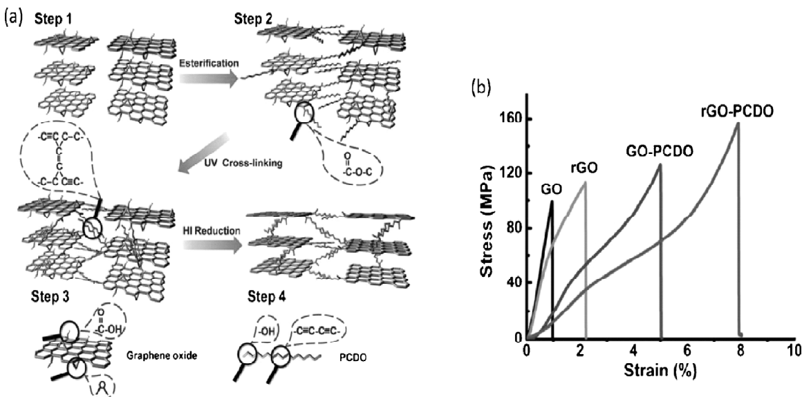
Figure 11: Schemes of the esterification, crosslinking, and reduction from the graphene oxide nanocomposites and corresponding changes of mechanical properties [112]. Copyright 2013. Reproduced with permission from John Wiley & Sons Inc.
