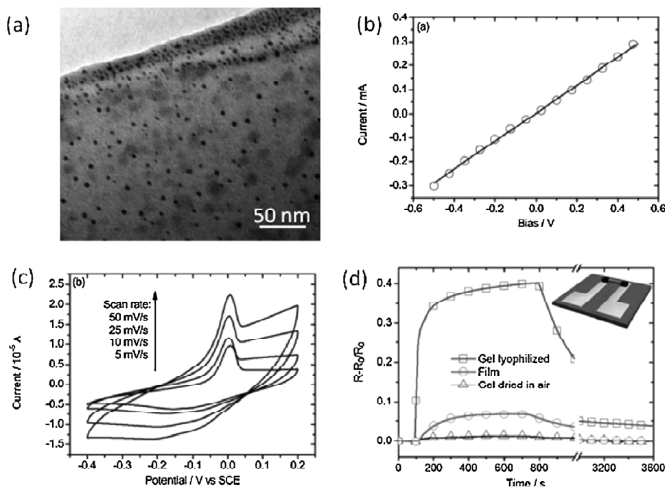
Figure 21: (a) TEM of a GO/PPy nanocomposite sheet with platinum nanoparticles embedded, (b) I-V curve of a lyophilized GO/PPy hydrogel, (c) cyclic voltammograms of GO/PPy hydrogel in 0.1 M LiClO 4 at different scan rates, and (d) Ammonia gas sensing performance of three devices with different sensing elements [230]. Copyright 2011. Reproduced with permission from the Royal Society of Chemistry.
