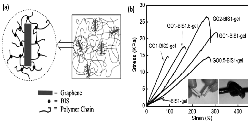
Figure 20: (a) Scheme of the crosslinked gel network consists of graphene, BIS, and PAA; (b) stress-strain curves of PAA gels with different combinations of GO and BIS contents. The inset shows the photographs of BIS-gel and GO-BIS gel from left to right, respectively [223]. Copyright 2012. Reproduced with permission from the Royal Society of Chemistry.
