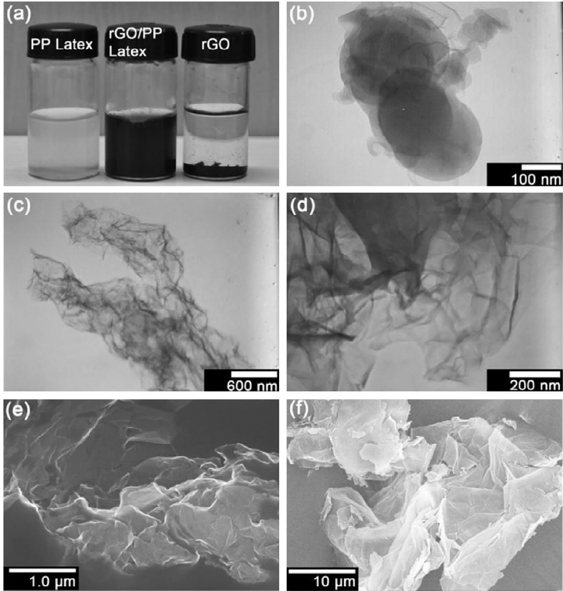
Figure 5: (a) Aqueous suspensions of PP latex and graphene oxide. (b) TEM image of PP latex. (c) and (d) TEM images of the rGO/PP latex composite dispersed in water before filtration. (e) SEM image of fracture surface of the rGO/PP composite (after hot-press molding). (f) SEM of agglomerated rGO nanosheets [161].
