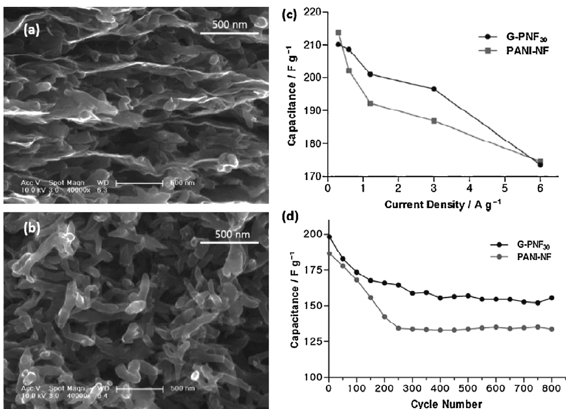
Figure 24: Cross-section SEM images of (a) pure chemically converted graphene and (b) graphene-PANI nanofiber composite film. (c) Plot of specific capacitance versus current density of graphene-PANI composite and PANI, and (d) cycling stability of graphene-PANI composite and PANI films [155]. Copyright 2010. Reproduced with permission from the American Chemical Society.
