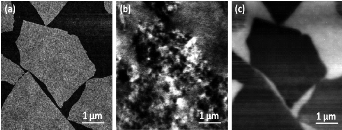
Figure 3: (a) Topography, (b) EFM-phase image before reduction, and (c) after chemical reduction from the same graphene oxide flakes.
