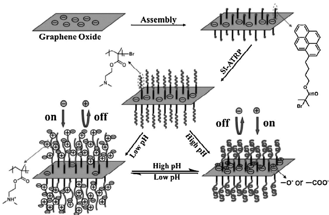
Figure 7: The preparation from PDMAEMA-modified graphene oxide and charging state of the GO-g-PDMAEMA composite at different pH values [170]. Copyright 2013. Reproduced with permission from John Wiley & Sons Inc.
