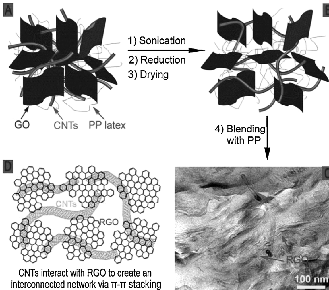
Figure 6: (A) and (B) The formation from interconnected network of rGO and CNTs using PP latex as a dispersing agent. (C) TEM image of PP/RGO/CNTs ternary system. (D) Schematic of strong interactions between RGO and CNTs via stacking [169]. Copyright 2013. Reproduced with permission from the Institute of Physics.
