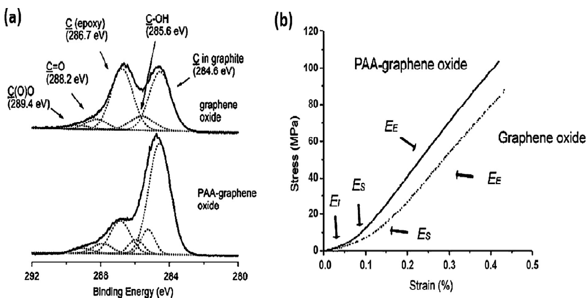
Figure 13: (a) XPS spectra of the graphene oxide paper and the PAA modified graphene oxide paper, showing effective chemical crosslinking; (b) stress-strain curves of the PAA modified and pristine graphene oxide papers, respectively [97]. Copyright 2009. Reproduced with permission from the American Chemical Society.
