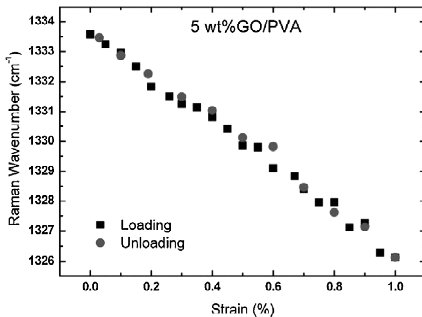
Figure 17: Shift of the D band position with strain to the PVA-graphene oxide nanocomposite for loading and unloading [210]. Copyright 2013. Reproduced with permission from the American Chemical Society.
