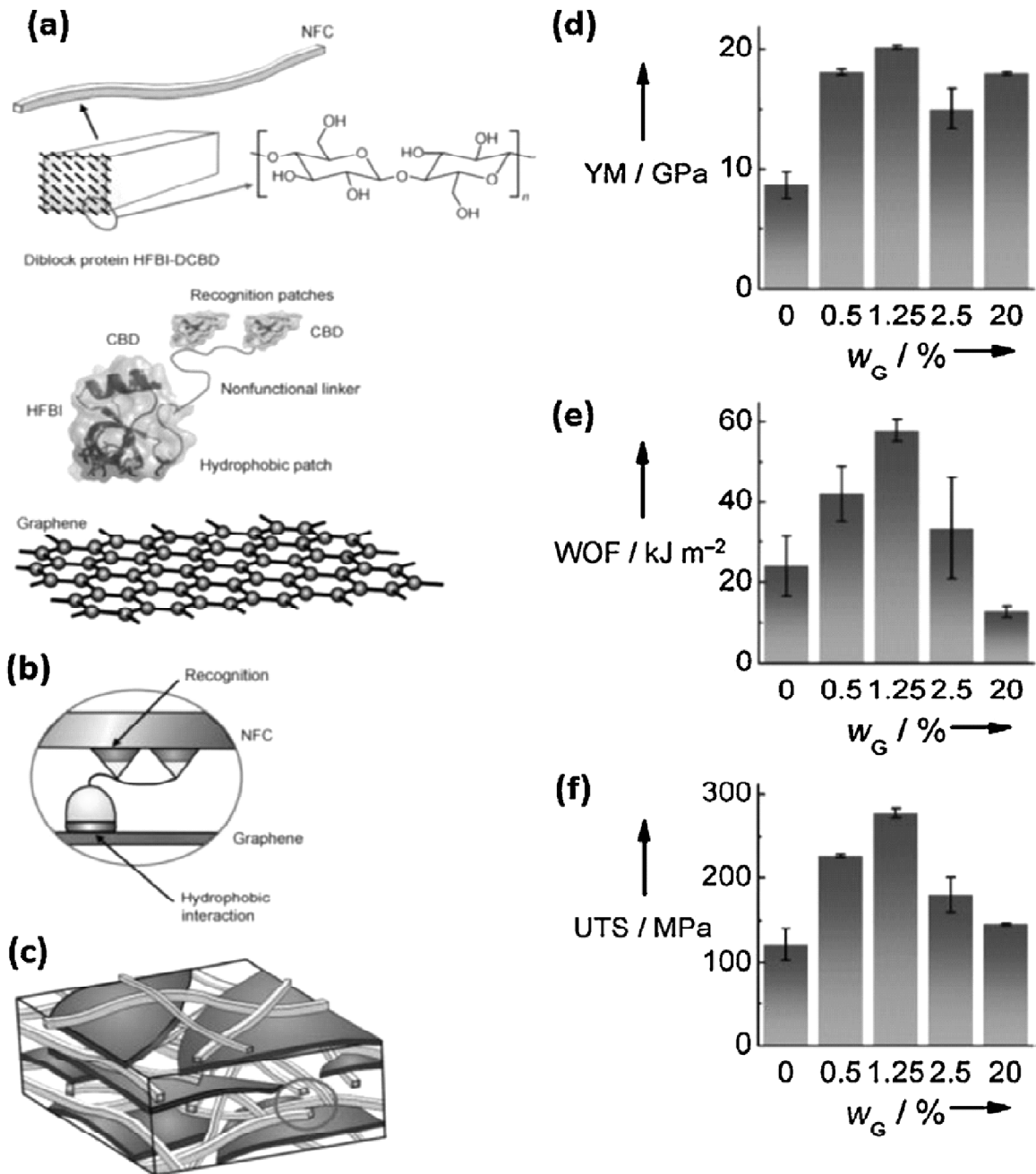
Figure 19: (a)–(c) The assembly of the graphene-NFC nanocomposites; (d)–(f) mechanical properties of the graphene nanocomposites: Young's modulus (YM), work of fracture (WOF), and ultimate tensile stress (UTS) versus the weight fraction from graphene in the nanocomposite, respectively [214]. Copyright 2011. Reproduced with permission from John Wiley & Sons Inc.
