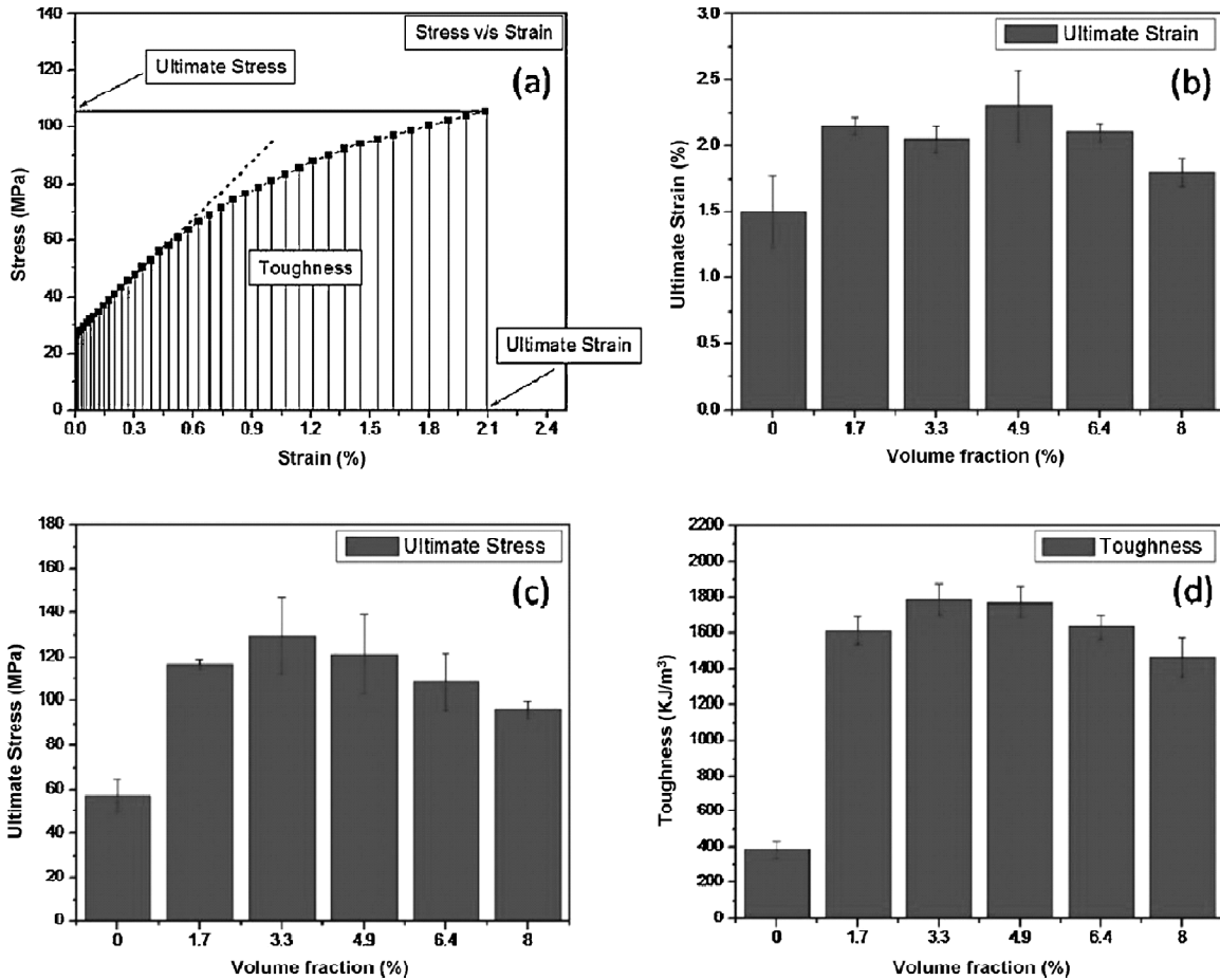
Figure 15: Representative stress–strain curve (a) of the graphene oxide-polyelectrolyte nanomembranes and the effect of graphene oxide content on the mechanical properties: (b) ultimate strain, (c) ultimate stress, and (d) toughness [3]. Copyright 2010. Reproduced with permission from the American Chemical Society.
