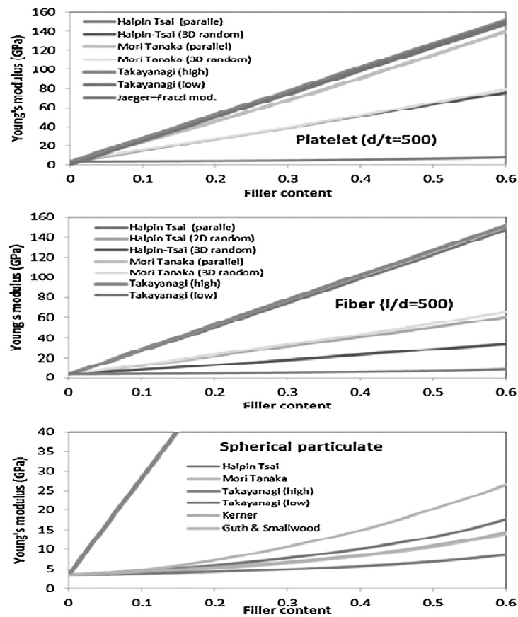
Figure 4: Calculations of the theoretical values of elastic modulus predicted by different models described above with the elastic modulus of 150 GPa and 3.5 GPa, and Poisson's ratio of 0.25 and 0.4 for the filler and the matrix, respectively.
