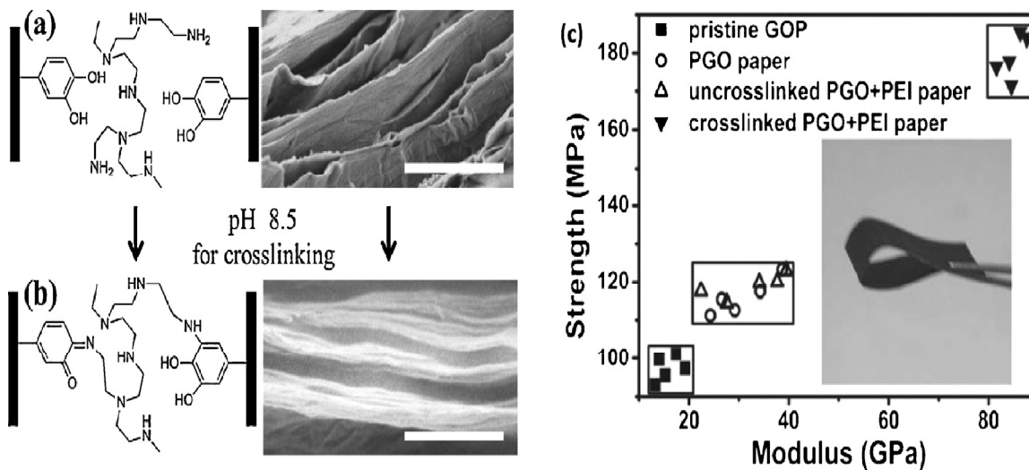
Figure 14: The chemical structure and SEM morphologies of the graphene oxide paper before (a) and after (b) PEI crosslinking. (c) Summary of the mechanical performance of the PEI crosslinked graphene oxide paper [208]. Copyright 2013. Reproduced with permission from John Wiley & Sons Inc.
