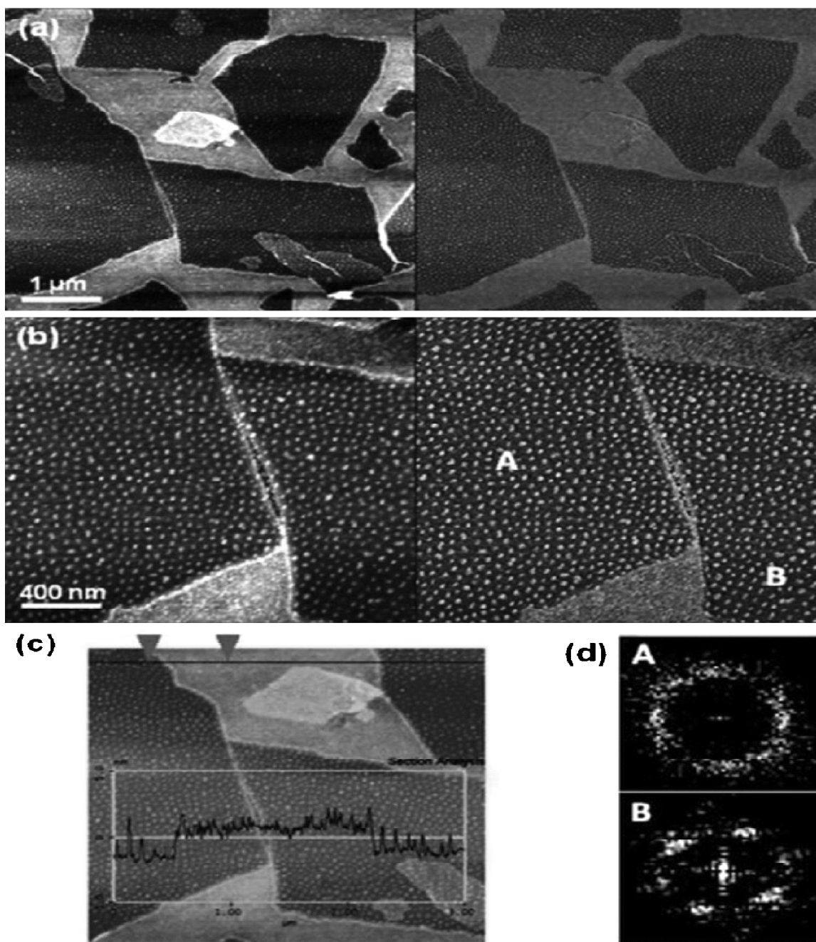
Figure 9: AFM topography (left) and phase (right) of (a and b) GO/PS 28 P2VP 28 star copolymer at pH 2 for surface pressures of 15 mN/m; (c) the height profile of corresponding topography image; (d) FFT of domain morphologies for A and B regions from Fig. 10b. z-scale: 5 nm (topography) and 30° (phase) [192]. Copyright 2013. Reproduced with permission from the American Chemical Society.
