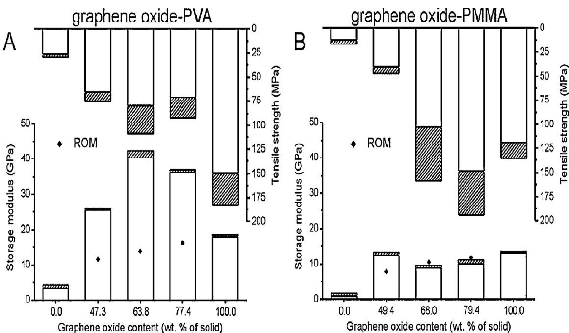
Figure 16: Storage moduli and tensile strengths of: (A) PVA-based and (B) PMMA-based nanocomposites. The average and maximum values are shown by the white and shaded bars, respectively [209]. Copyright 2010. Reproduced with permission from John Wiley & Sons Inc.
