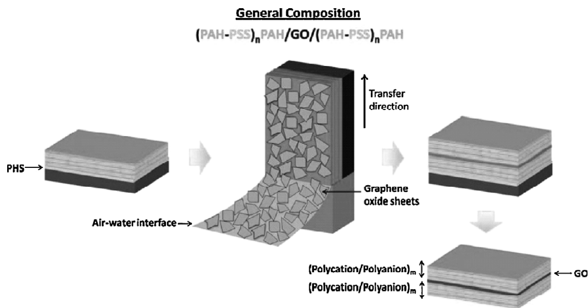
Figure 8: Fabrication from ordered and hierarchical multilayered graphene oxide-polyelectrolyte nanomembranes via combination from LBL and LB techniques [3]. Copyright 2010. Reproduced with permission from the American Chemical Society.
