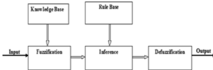
Figure 3: Fuzzy Logic Controller
