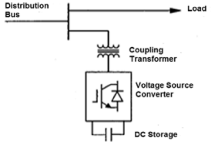
Figure 2: Block Diagram of Dstatcom
