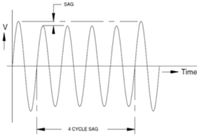
Figure 1: Graphical Representation of Voltage Sag
