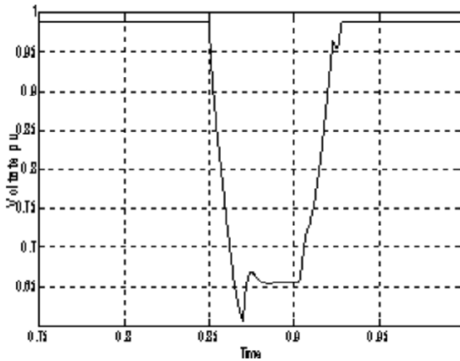
Figure 8: Output of the System without Dstatcom in the system
