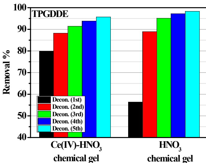
Figure 6: Removal percentage of uranium with the number of decontaminations for a Ce(IV)-HNO 3 & HNO 3 solution containing a TPGDDE coviscosifier.
