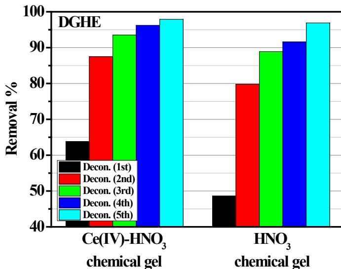
Figure 4: Removal percentage of uranium with the number of decontaminations for a \text{Ce(IV)-HNO}_3 & \text{HNO}_3 solution containing a DGHE coviscosifier.
