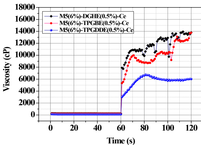
Figure 3: Rheogram of various chemical gels: shearing for 60s at a shear rate of 500/s followed by a shearing for 60s at 5/s.
