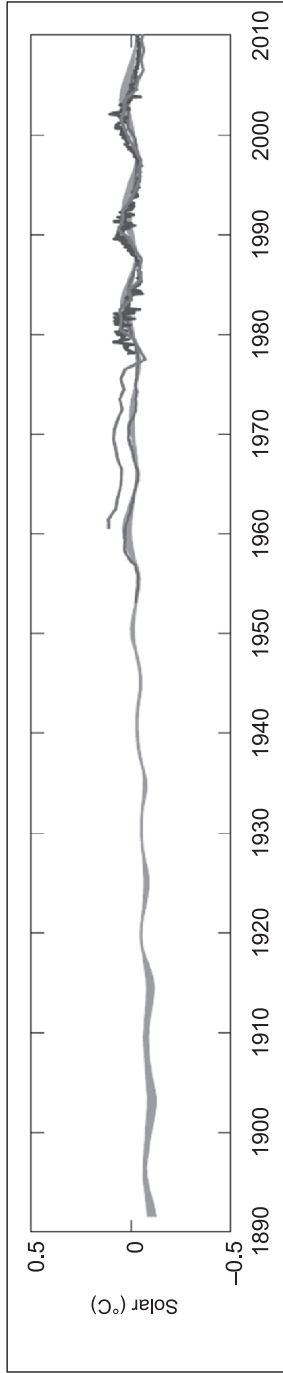
Figure 1: (c) Estimated trend of contribution of solar in global mean surface temperature
