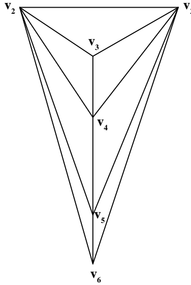
Figure 1: P\ell_6
