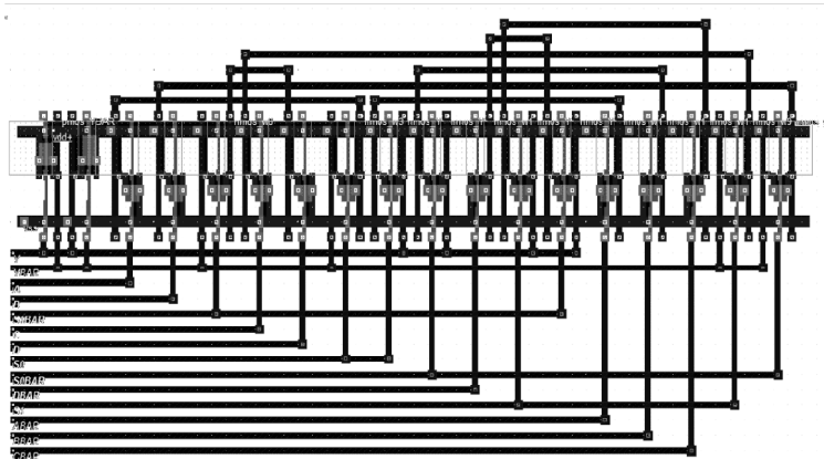
Figure 13: Layout diagram of Cascode voltage switch logic (CVSL) 4:1 multiplexer
