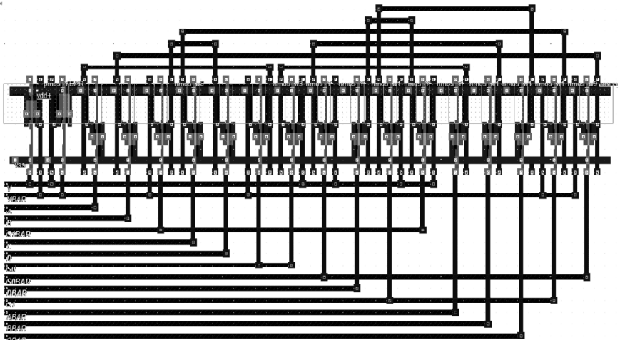
Figure 12: Layout diagram of positive feedback adiabatic logic (PFAL) 4:1 multiplexer
