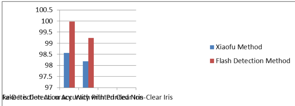
Fig. 4 : Comparison of proposed system with Xiaofu method
