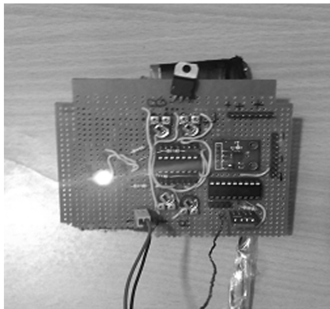
Figure 3: Hand gesture circuit with accelerometer and transmitter
