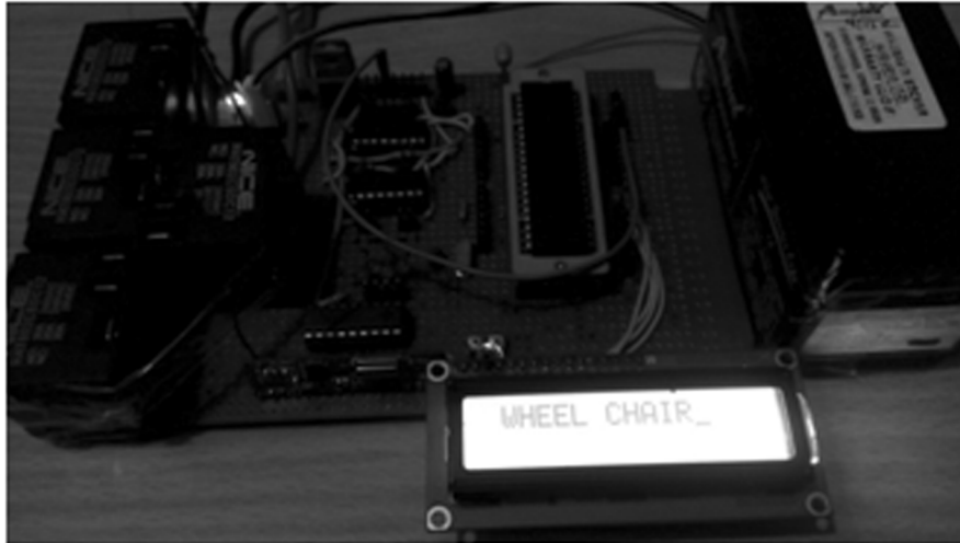
Figure 1: Receiver circuit of wheel chair with control unit
