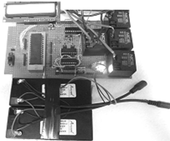
Figure 5: Overall circuit of wheelchair that controls the motion of motor
