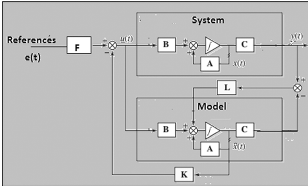
Figure 6: Observed state feedback optimal control
