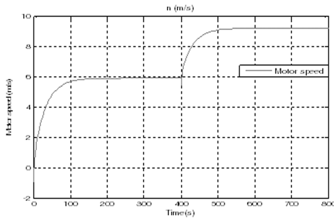
Figure 14: Motor speed
