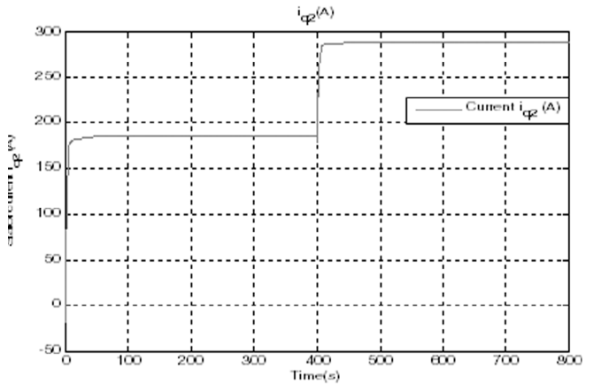
Figure 13: Stator current i_{q2}
