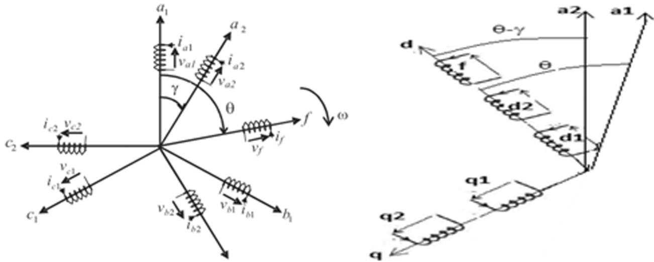
Figure 2: MSDE Machine and Park MSDE representation, with \gamma = 30^\circ
