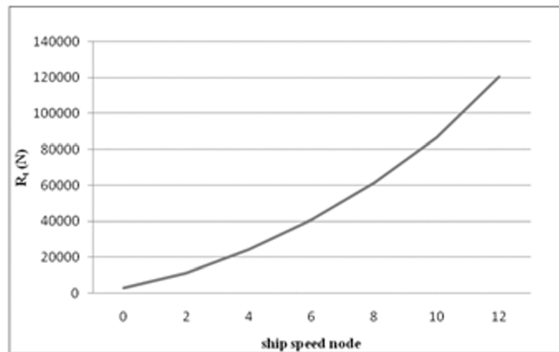
Figure 3: Hull resistance
