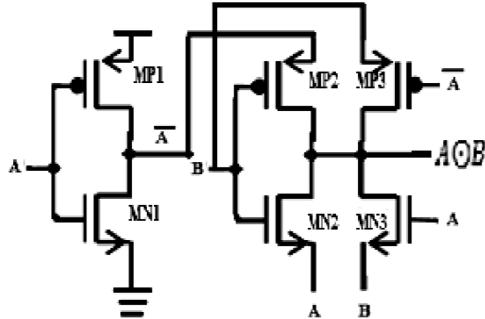
Figure. 2 XNOR module
