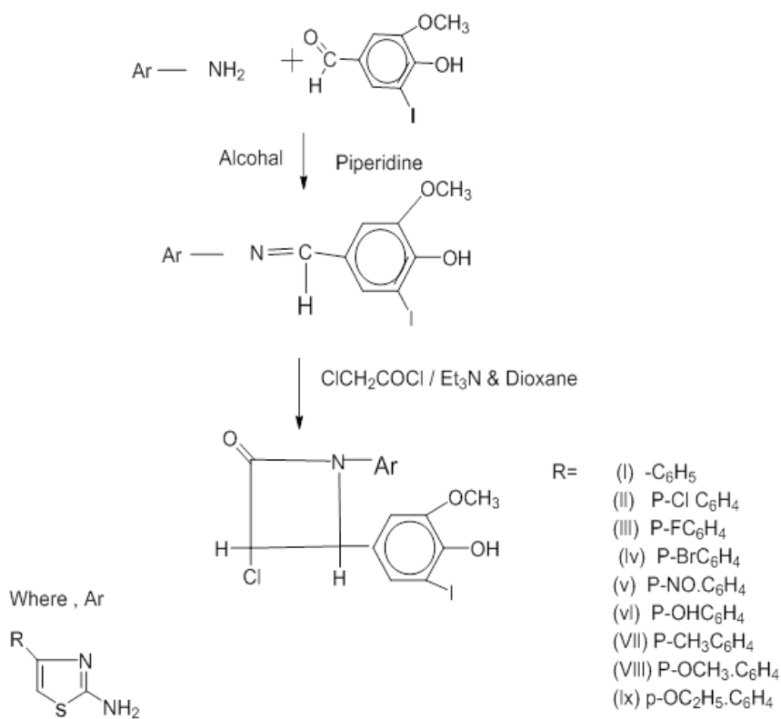
2-Amino-4-(P-subst / Un-subst)-phenyl thiazole
