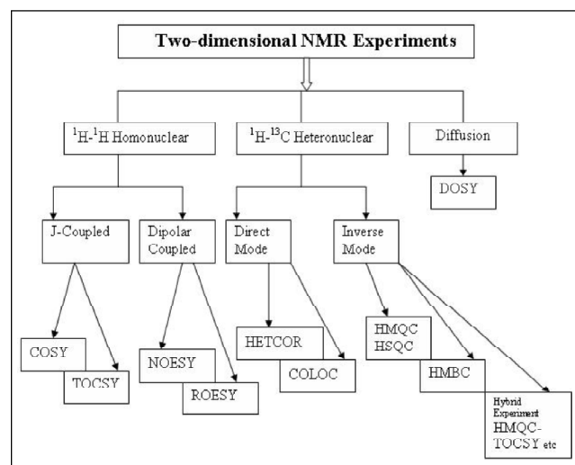
Figure 2: Flowchart for two dimensional NMR experiments
