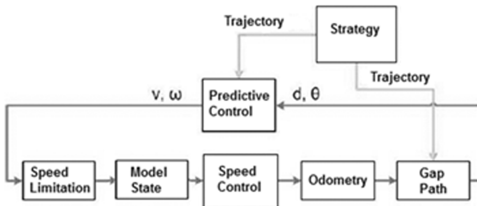
Figure 8: General functional regulation
