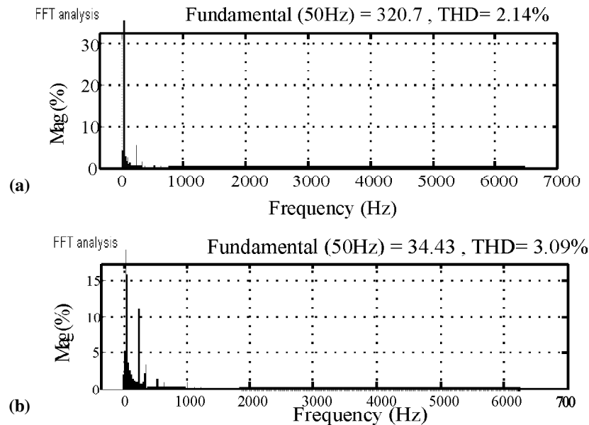
Figure 11: FFT analysis of the PMSG-based Hybrid wind energy system in varying wind as well as load conditions: (a) Load voltage, (b) Load current
