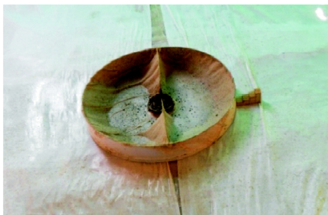
Figure 2: Modified Morgan's splash cup
