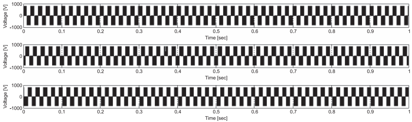
Figure 5: Two-level voltage source inverter line to line voltage
