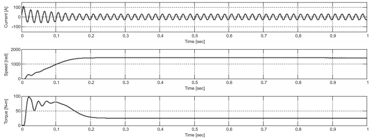
Figure 12: Three-phase Induction Motor Current, Speed and Torque
