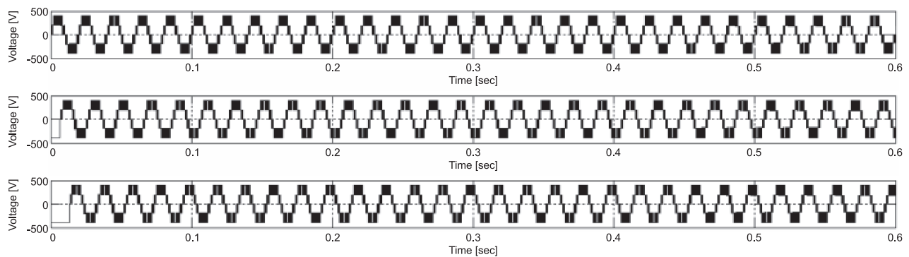
Figure 11: Five-level Inverter phase to phase Voltage
