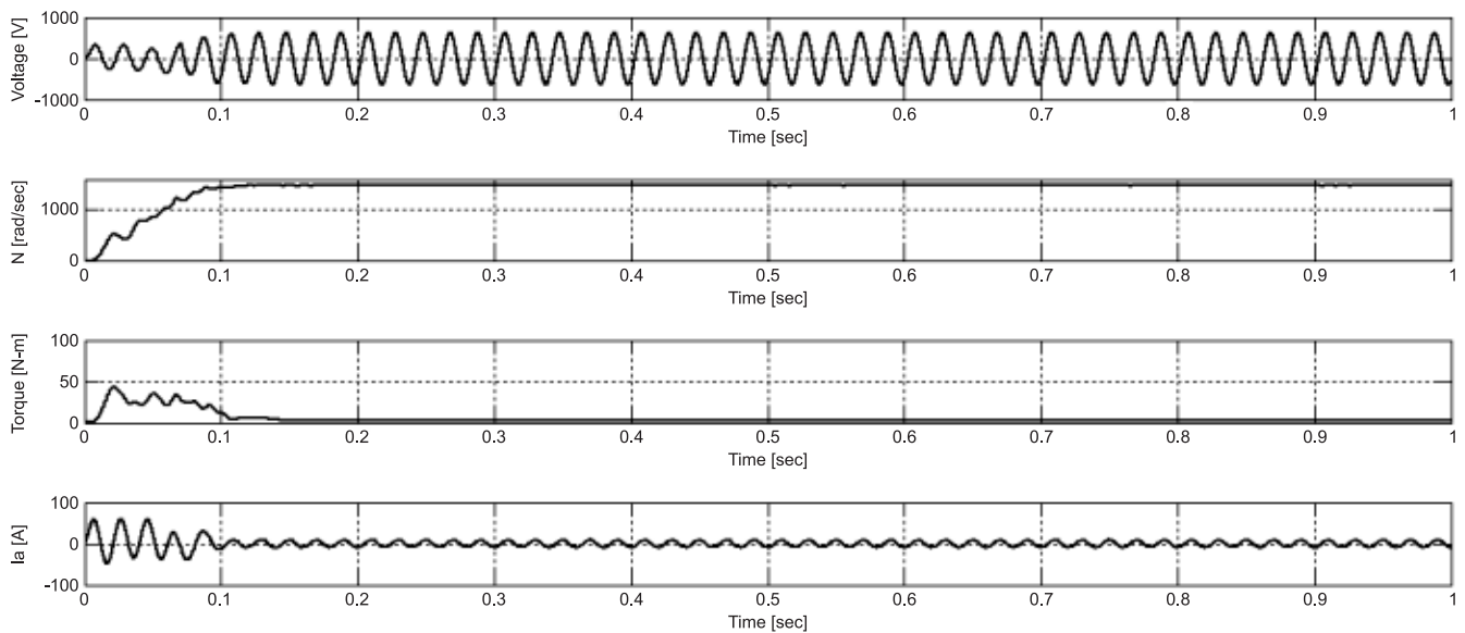
Figure 4: Single phase Induction Motor Voltage Capacitor, Speed, Torque and Winding Current
