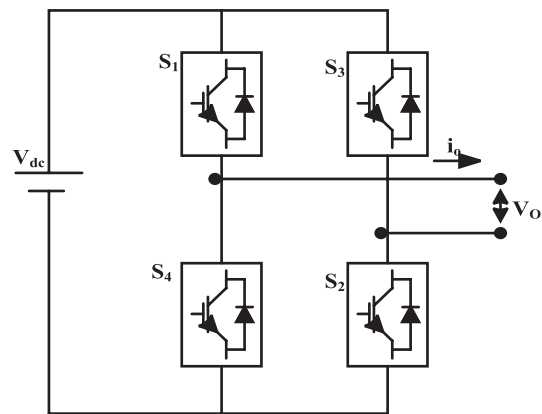
Figure 2: Single-Phase Full Bridge Inverter
