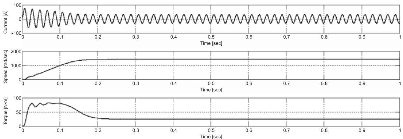
Figure 7: Three phase Induction Motor Current, Speed and Torque
