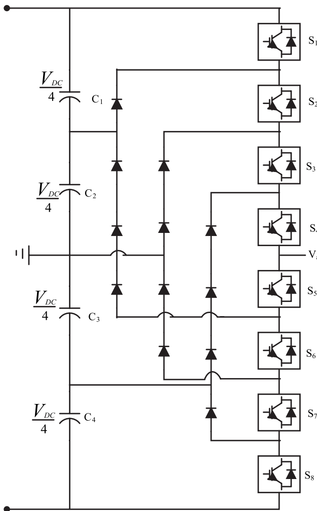
Figure 1: (a) 5-Level Diode Clamped MLI
