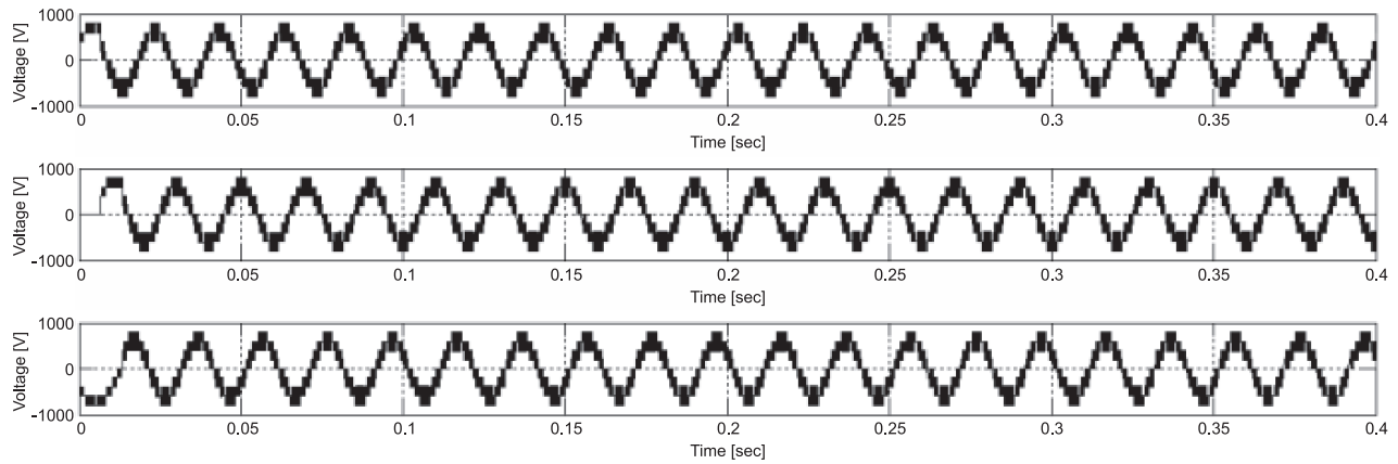
Figure 10: Five-Level Inverter line to line Voltage
