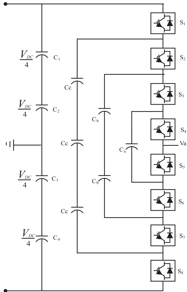
Figure 1: (b) 5-Level Flying-Capacitor MLI
