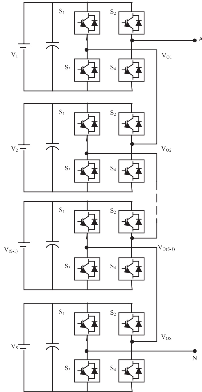
Figure 1: (c) 5-Level Cascaded MLI
