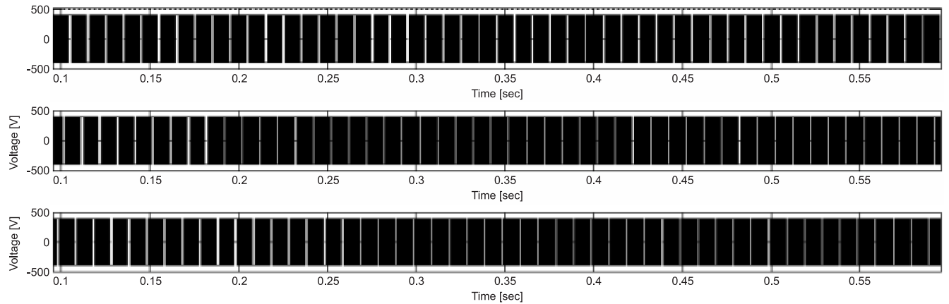
Figure 6: Two-level voltage source inverter phase to phase voltage
