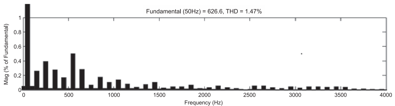
Figure 13: FFT analysis of 5-phase 5-level inverter
