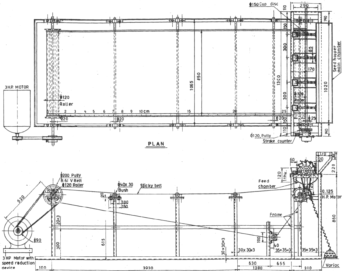
Figure 2: Test Rig for Performance Evaluation of Cup Feed Metering Device
