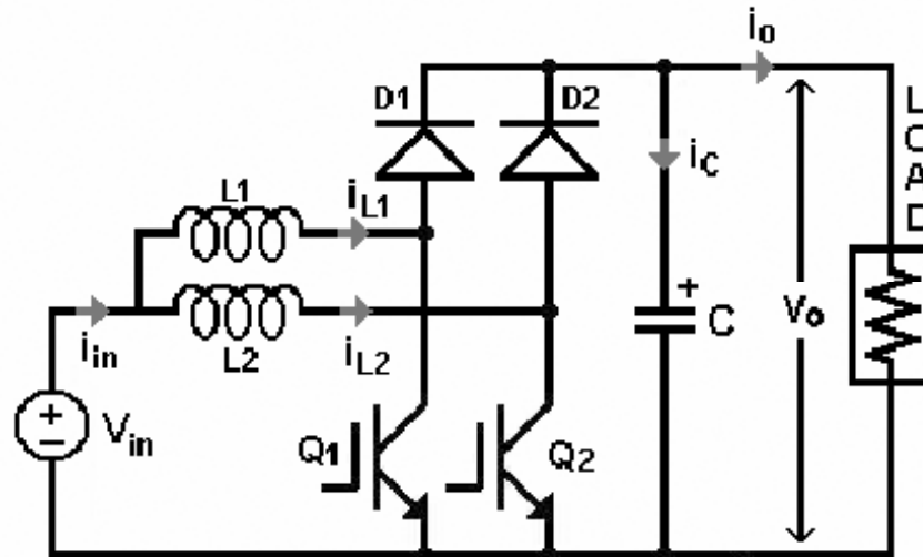
Figure 3: Interleaved Boost DC-DC Converter
