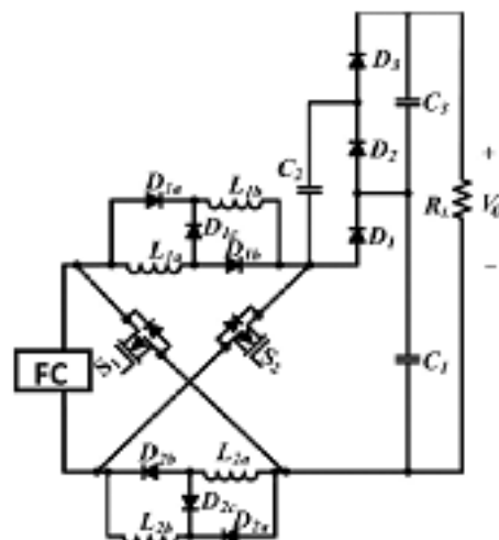
Figure 6: Proposed dc-dc converter
