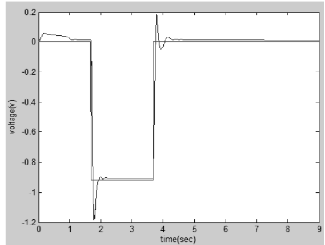
Figure 10: Response of compensated system for -0.6v step input
