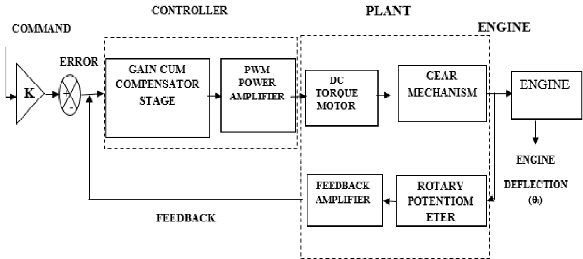
Figure 1: EGCS servo loop Block diagram including engine
