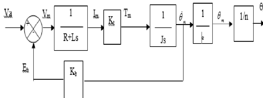
Figure 4: Block diagram of electro-mechanical actuator
