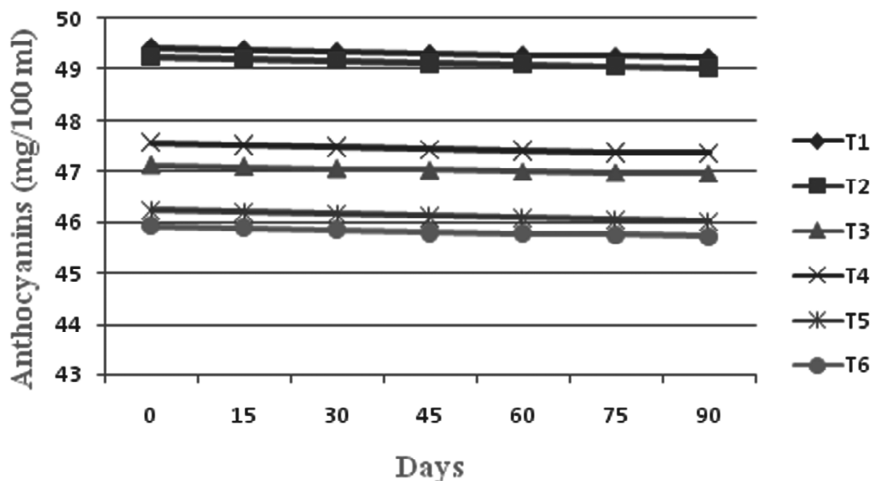
Figure 3: Changes in anthocyanins (mg/100 ml) of jamun and pomegranate juice blends as influenced by different treatments during storage period
