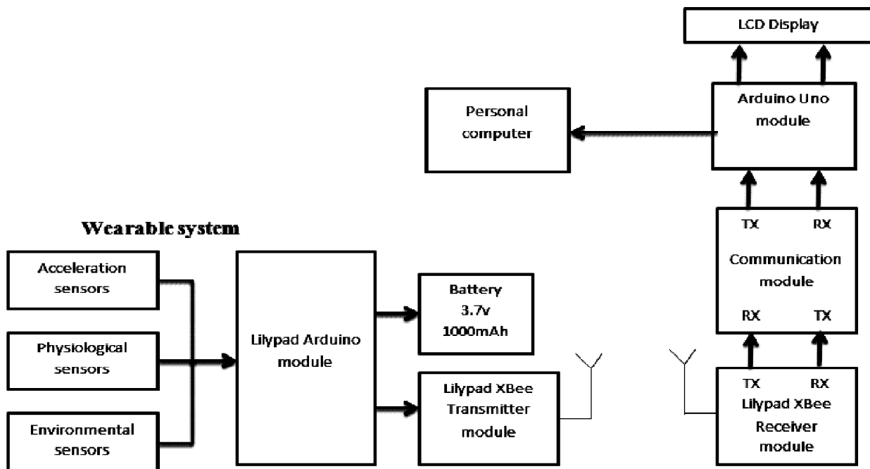
Figure 1: Data acquisition system for Human activity recognition
